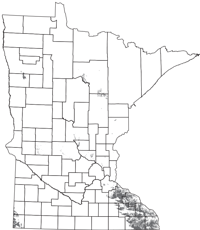
Figure 4. Eolian sand and loess coverage
