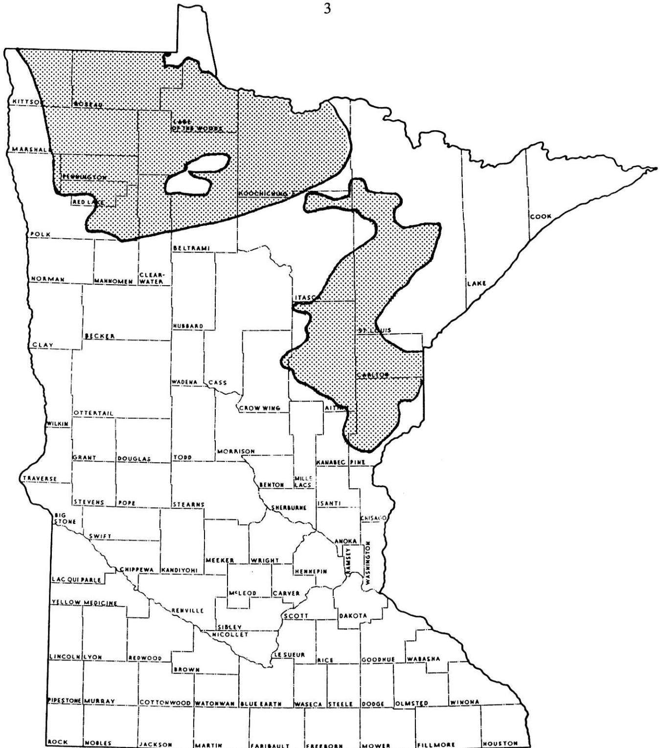
Figure 2. Northwest and east-central Minnesota sharp-tailed grouse ranges, 1995. Sharp-tails inhabit only scattered (usually disjunct) open landscapes in both ranges.
