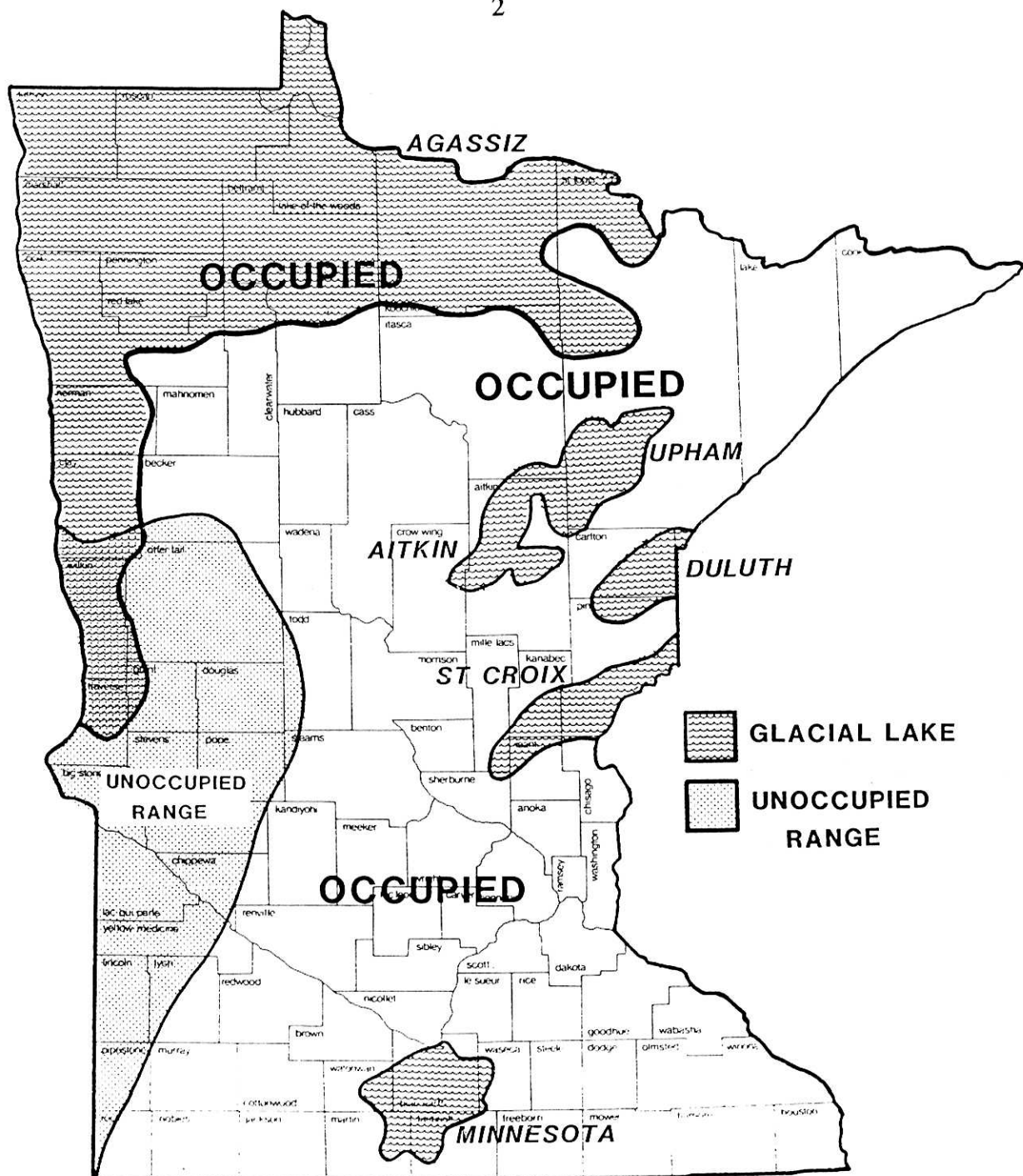
Figure 1. Pre-settlement (circa 1880's) distribution of sharp-tailed grouse in Minnesota in relation to the six major glacial lake beds (in italics). Glacial lake beds contained the larger peatlands which contain much of the present day sharptail range. Sharptails likely were not resident of the shaded area labeled "unoccupied range". Modified from Aldrich (1963).
