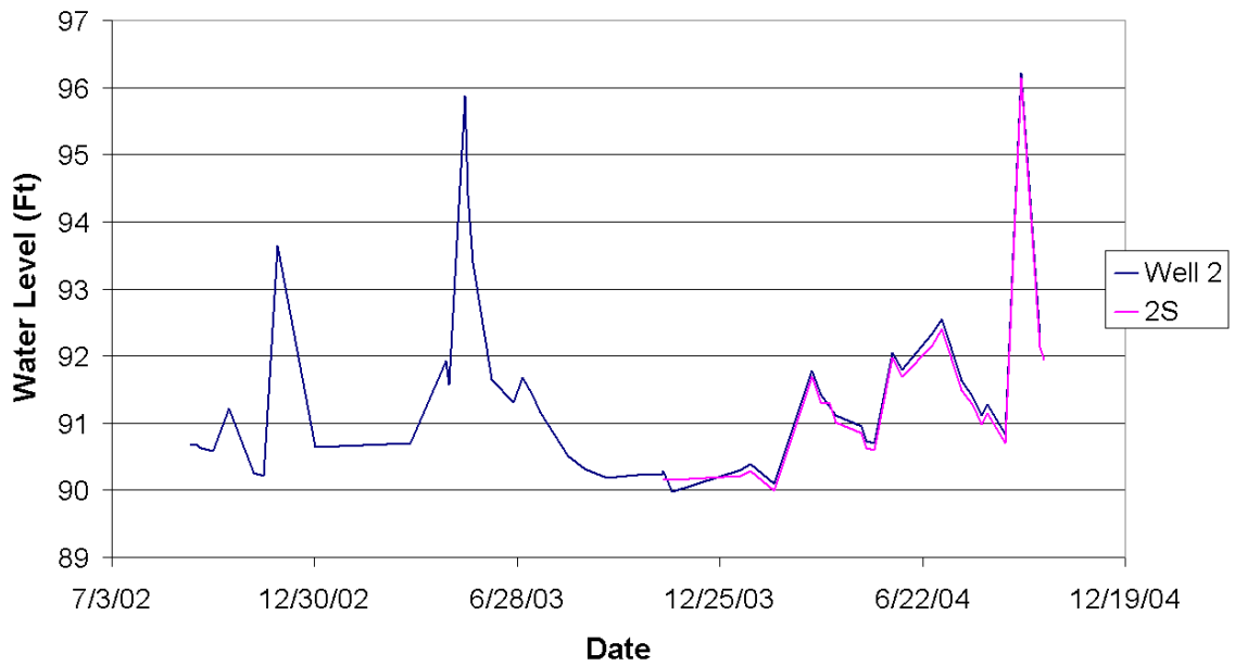
Figure 8.4b. Water levels, nest 2.
