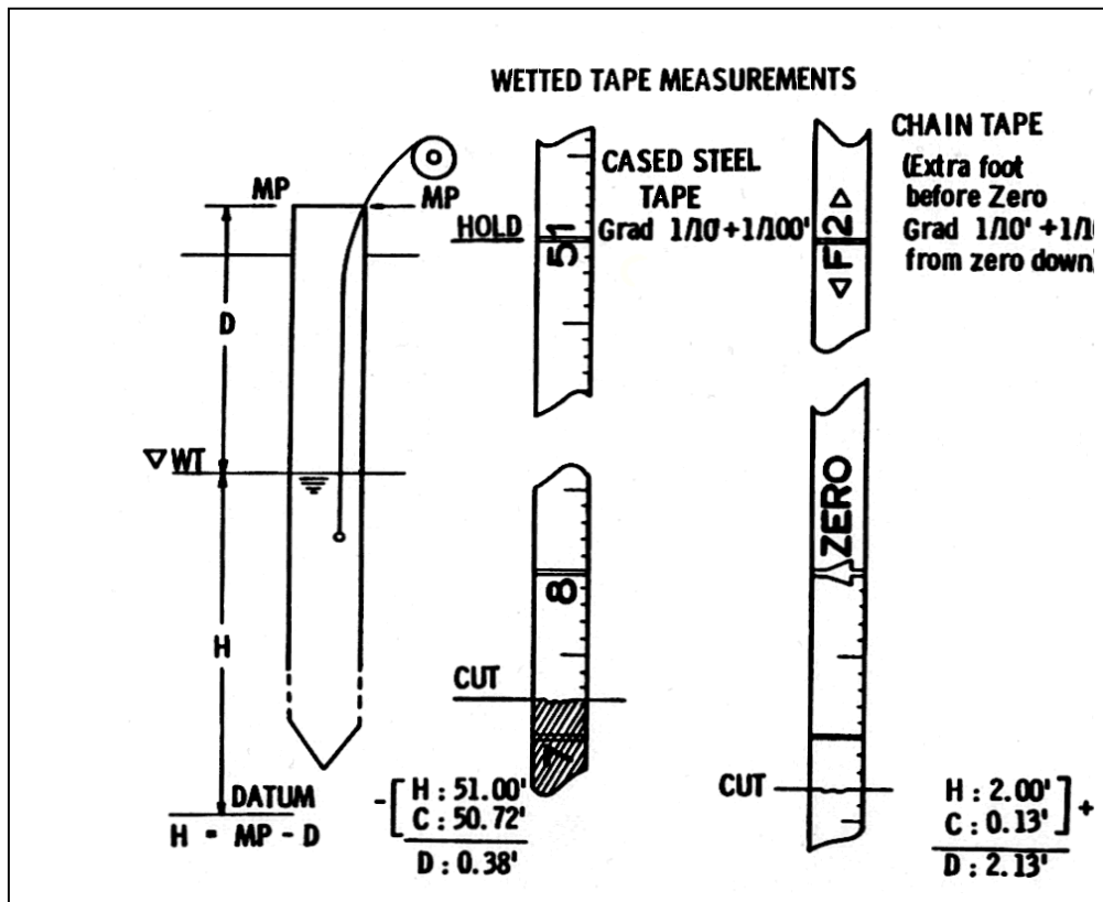
Figure 1. Steel tape.
