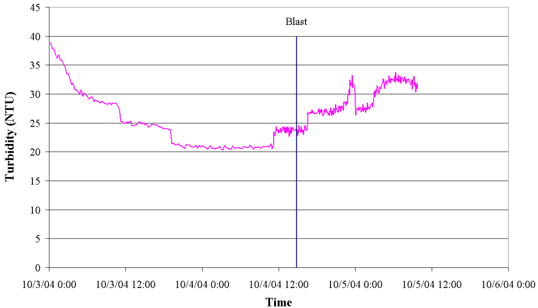
Figure 3. Monitoring showed slight turbidity increases after blasting at Fountain.
