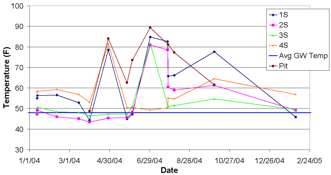
Figure 8.5. Fluctuations in ground-water temperatures.
