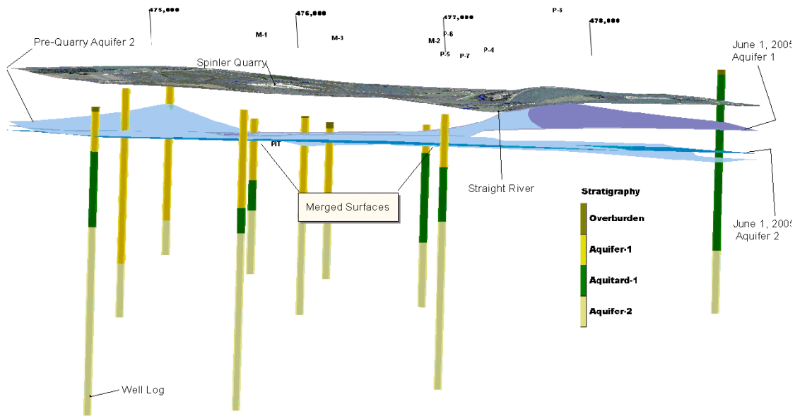
Figure 13. (vertical exaggeration 10:1)
