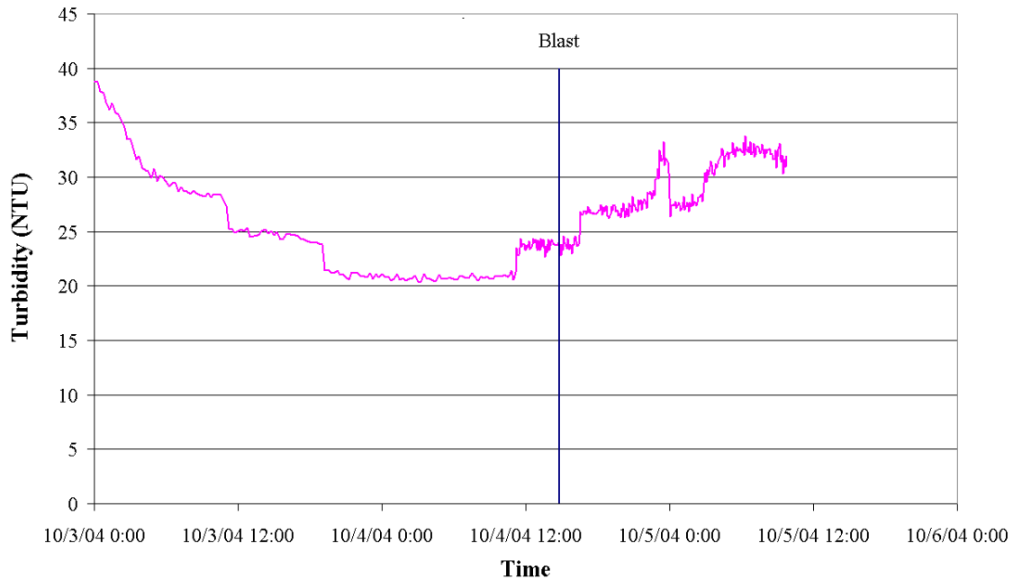
Figure 6.4. Fountain Big Spring turbidity after October 5, 2004 blast.
