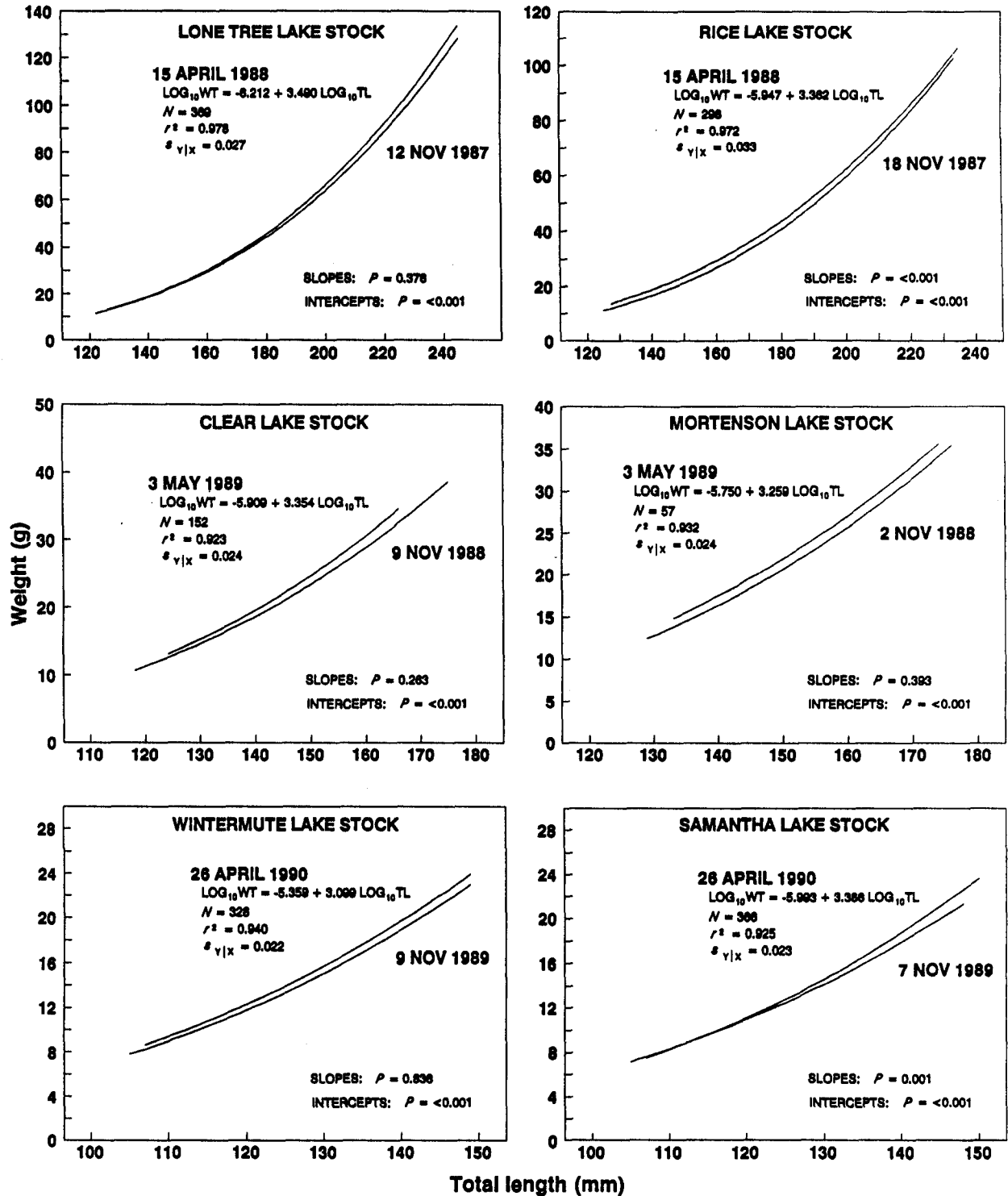
Figure 2. Weight-length curves of walleye fingerlings and pond-wintered yearlings, and results of Welch's t tests for equality of slopes and intercepts of scaled data. Lines were fitted by least-squares regression of \log_{10} transformed variables. Fingerling regression statistics are shown in Figure 1.
