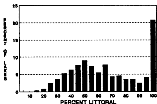
Figure 1. Frequency distribution (%) of percent littoral area for 3,029 classified lakes.
