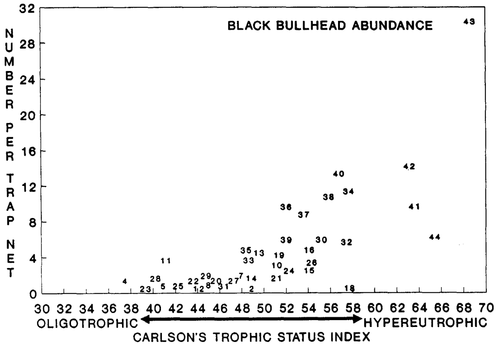
Figure 3. Median CPUE of yellow and black bullhead in lake survey trap nets for each lake class, and in relation to trophic status of the lake classes.
