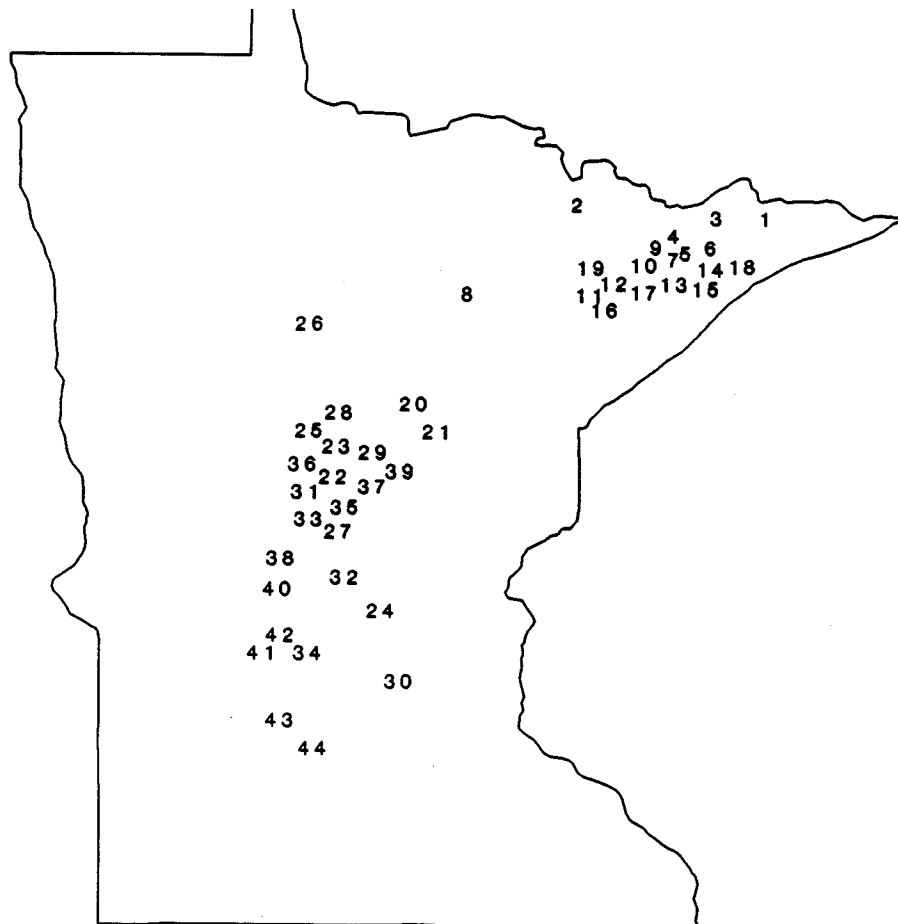
Figure 2. Approximate geographic centers of 44 lake classes.
