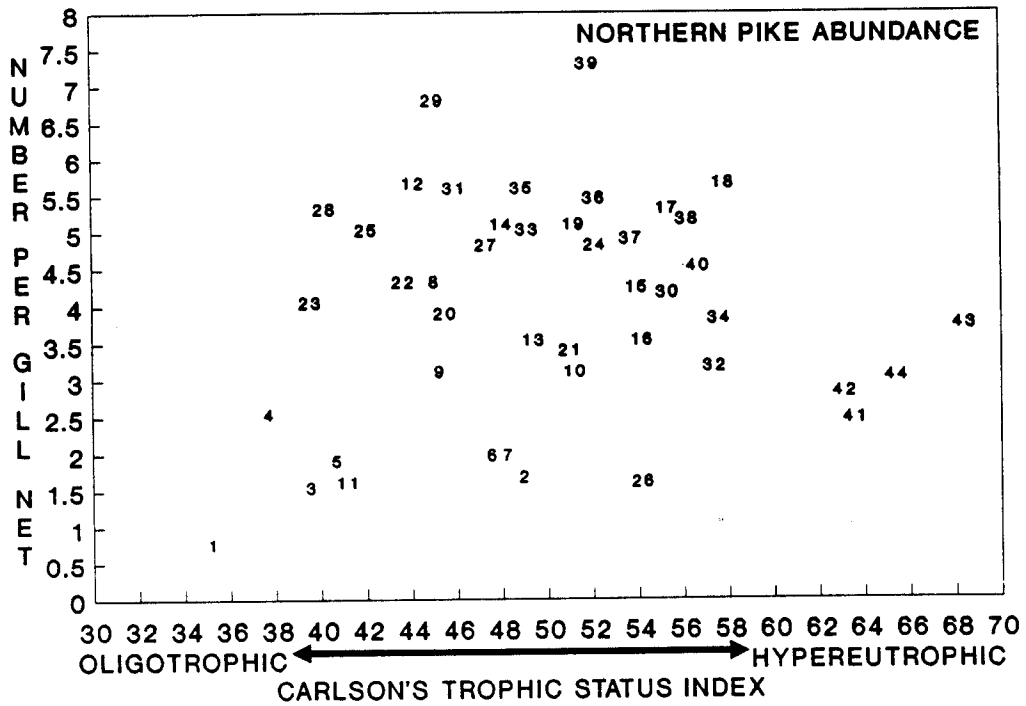
Figure 5. Median CPUE of white sucker and northern pike in lake survey gill nets for each lake class, and in relation to trophic status of the lake classes.
