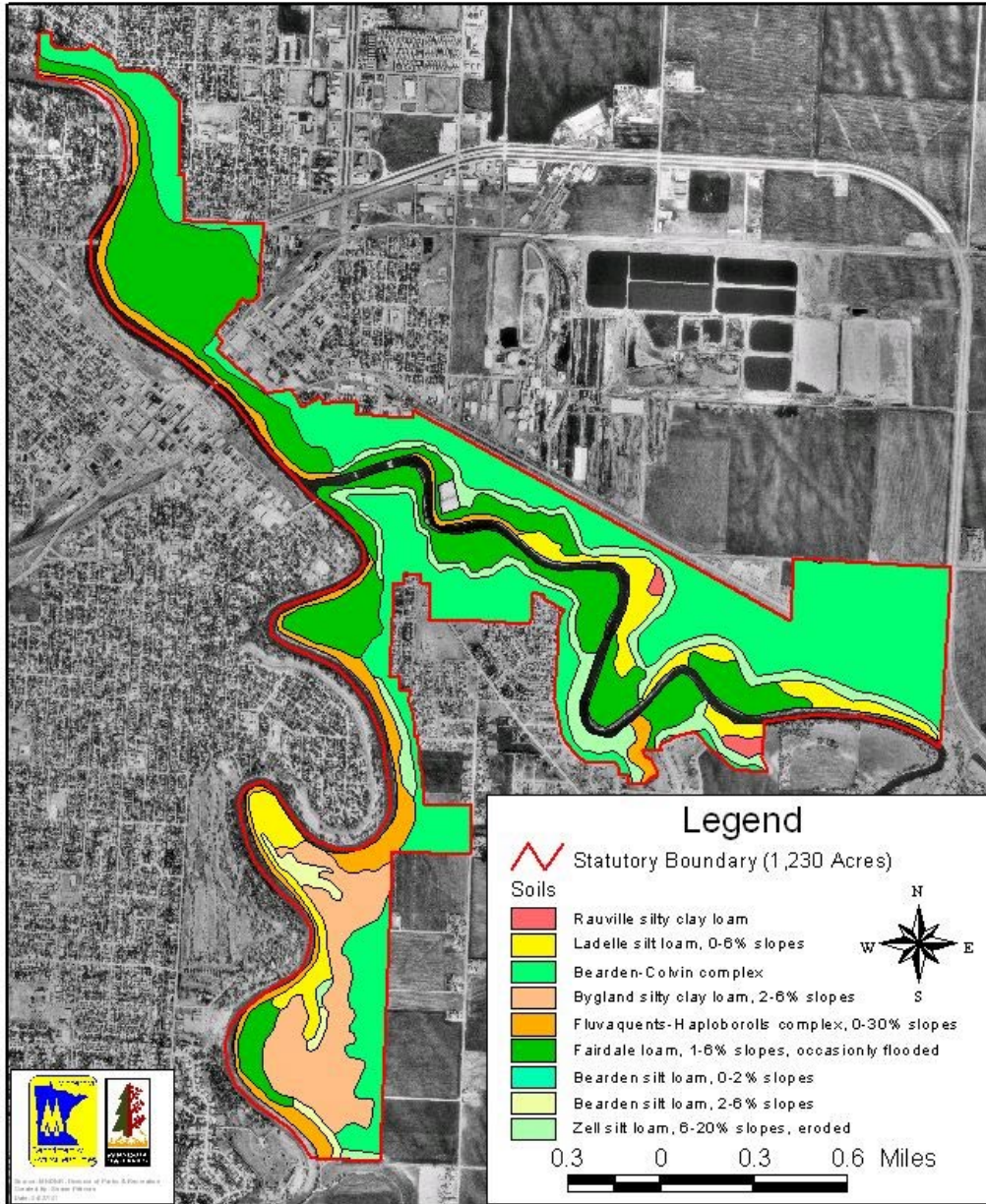
Figure 12: Red River State Recreation Area Soils
