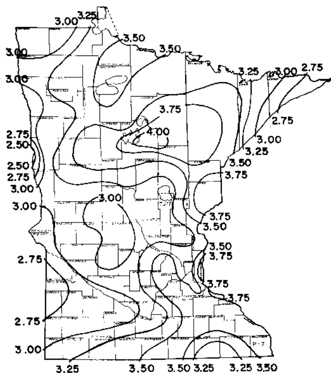
Figure 28. July normal precipitation in inches, Minnesota.
