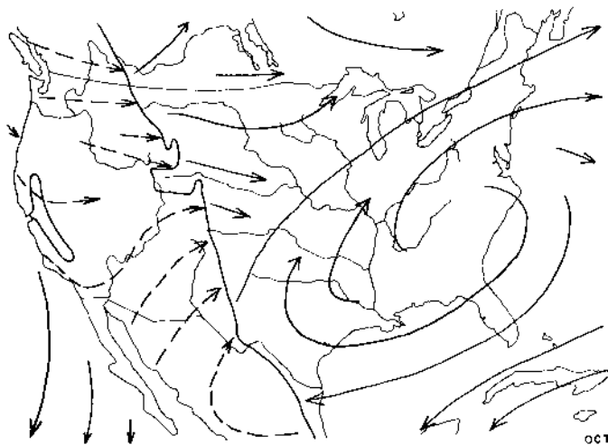
Figure 21. Resultant winds at 1,500 feet during October, United States. Anticyclonic winds centered over the southeastern United States now dominate most of the country from the Rockies eastward (3).
