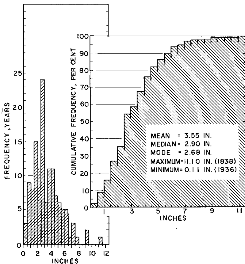
Figure 52. Frequency distribution and cumulative frequency distribution in inches of July precipitation in 1837-1965, Minneapolis-St. Paul.
