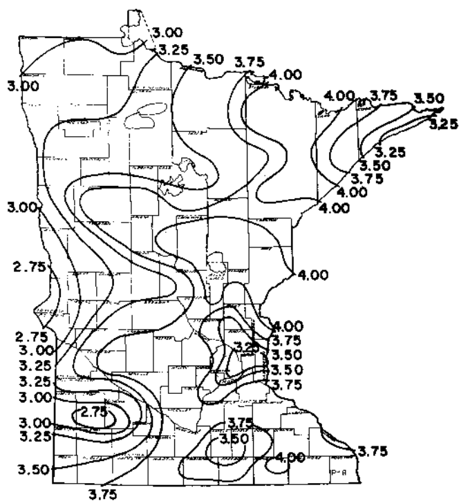
Figure 29. August normal precipitation in inches, Minnesota.
