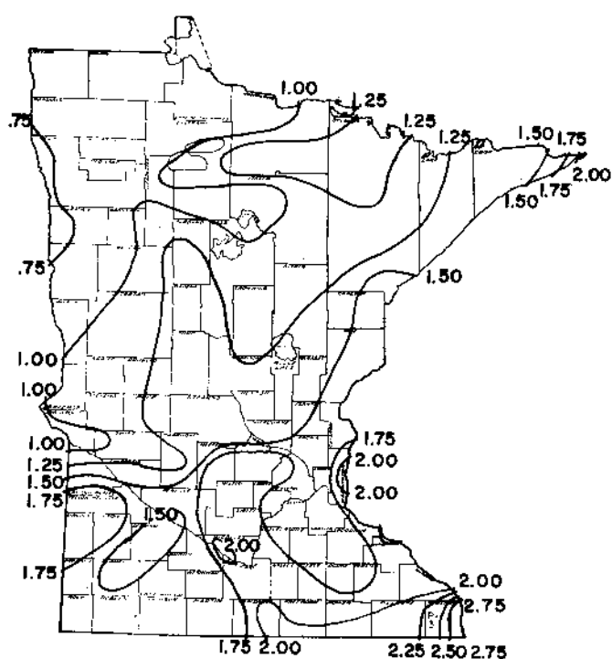
Figure 24. March normal precipitation in inches, Minnesota.
