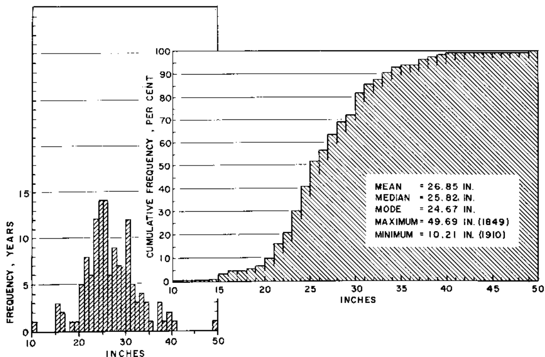
Figure 51. Frequency distribution and cumulative frequency distribution in inches of annual precipitation in 1837-1965, Minneapolis-St. Paul.
