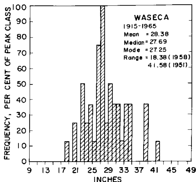
Figure 49. Distribution of annual precipitation in inches in 1915-65, Waseca. Distribution is expressed as a percent of the peak precipitation class.
