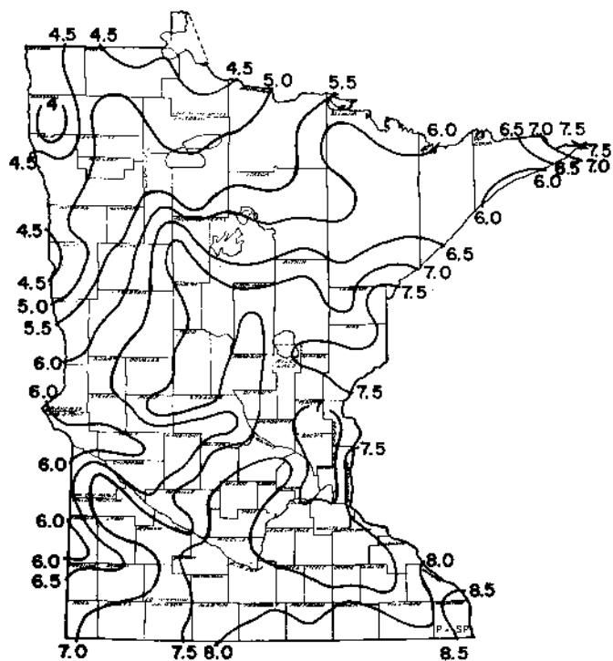
Figure 35. Spring (March, April, and May) normal precipitation in inches, Minnesota.
