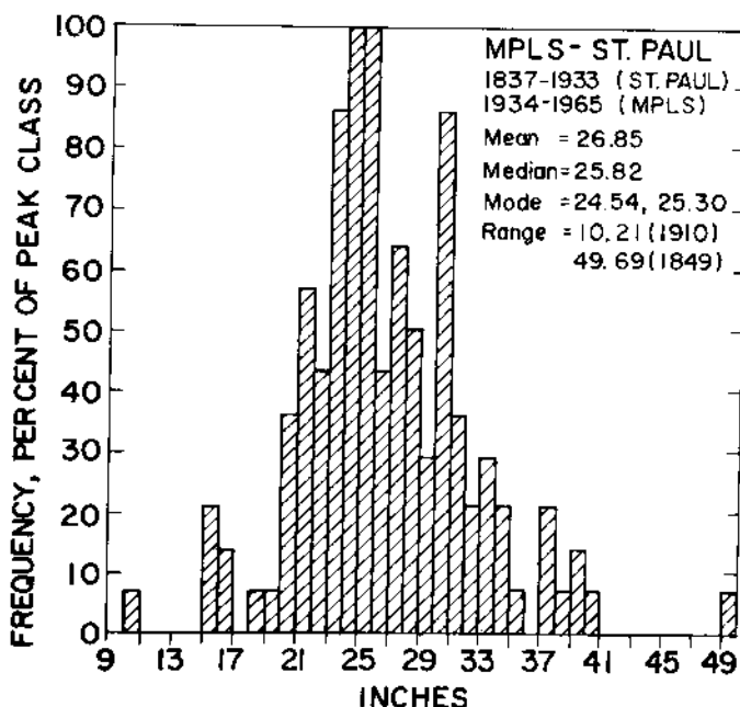
Figure 46. Distribution of annual precipitation in inches in 1837-1965, Minneapolis-St. Paul. Distribution is expressed as a percent of the peak precipitation class.
