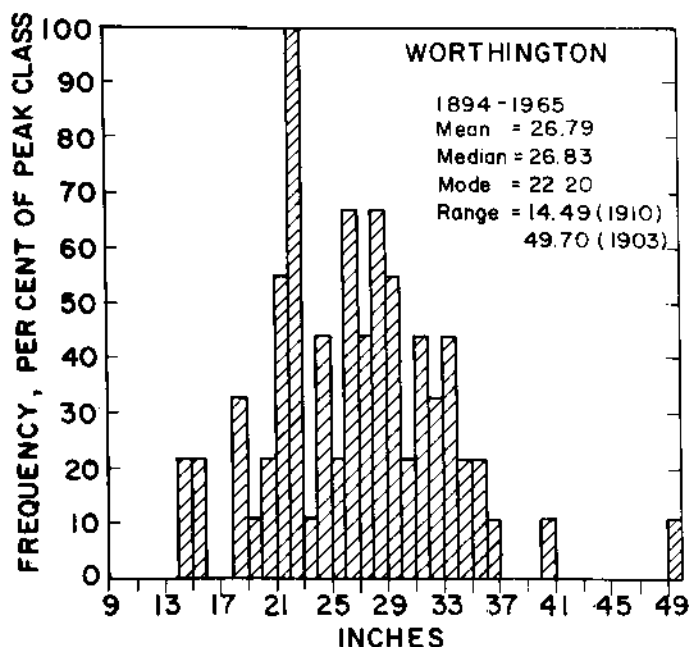
Figure 50. Distribution of annual precipitation in inches in 1894-1965, Worthington. Distribution is expressed as a percent of the peak precipitation class.
