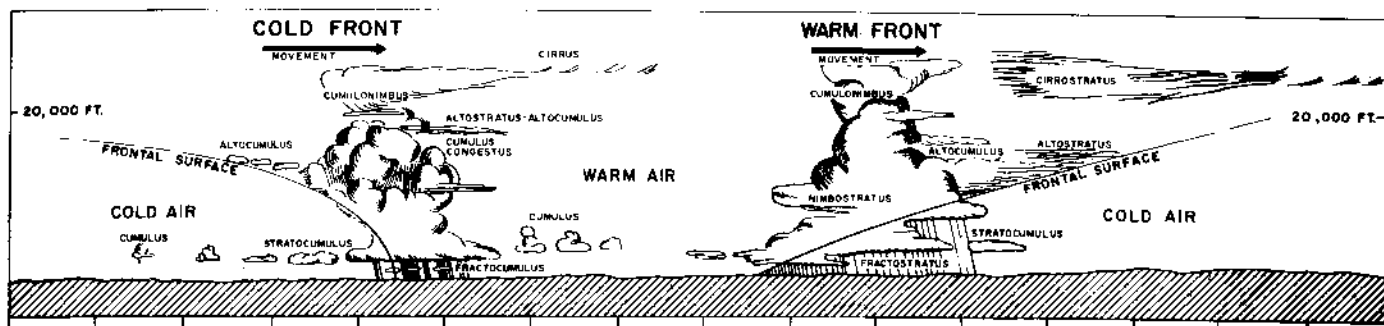
Figure 2. A cross section of a classical frontal system showing the types of clouds associated with it. The vertical, short tic marks at the bottom represent distances of about 100 miles. The vertical scale is greatly exaggerated.
