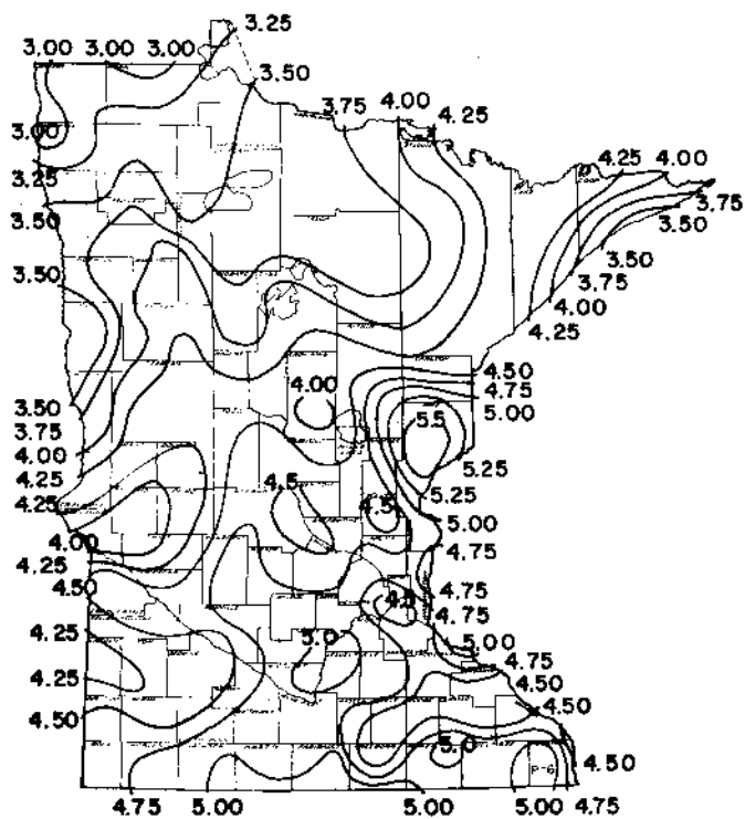
Figure 27. June normal precipitation in inches, Minnesota.
