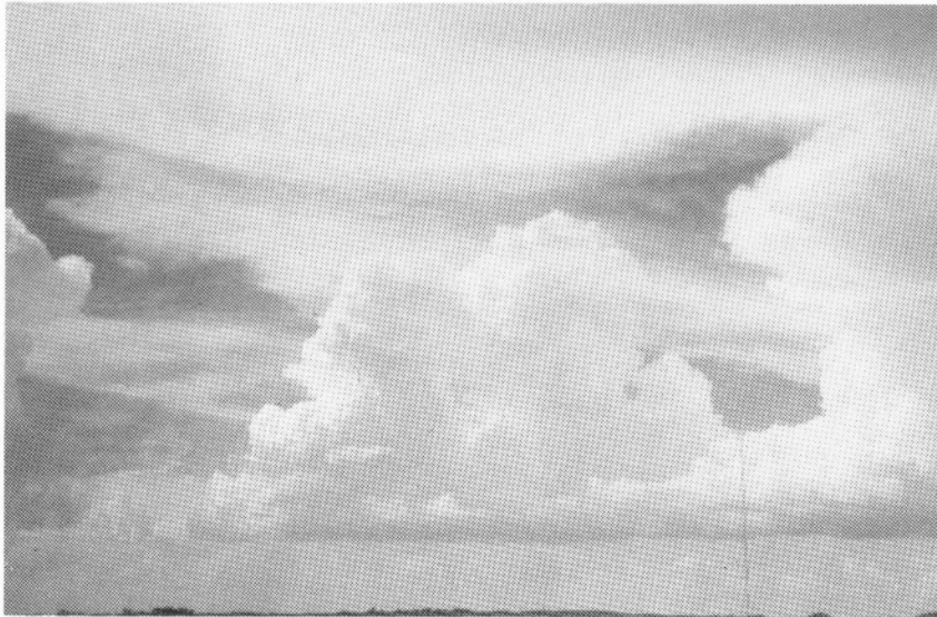
Figure 10. A towering cumulus cloud in the form of domes. It is accompanied by other cumulus at the same base level and dense cirrus at a much higher level. To its right, this same type of cloud is changing to the cumulonimbus (thunder-head) stage. (Collection of the authors)
