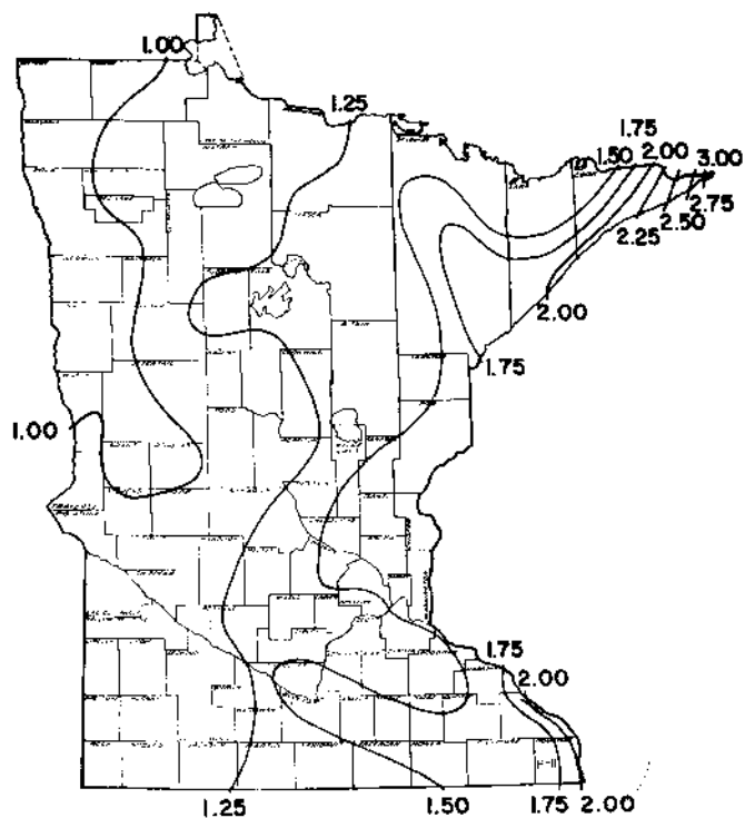
Figure 32. November normal precipitation in inches, Minnesota.
