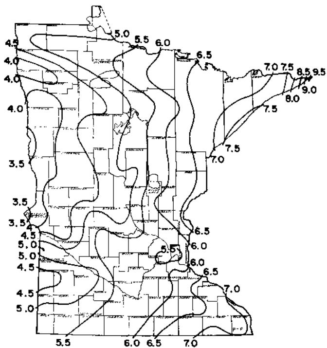
Figure 37. Fall (September, October, and November) normal precipitation in inches, Minnesota.
