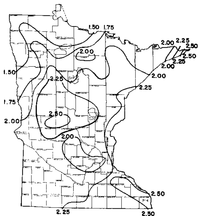
Figure 25. April normal precipitation in inches, Minnesota.
