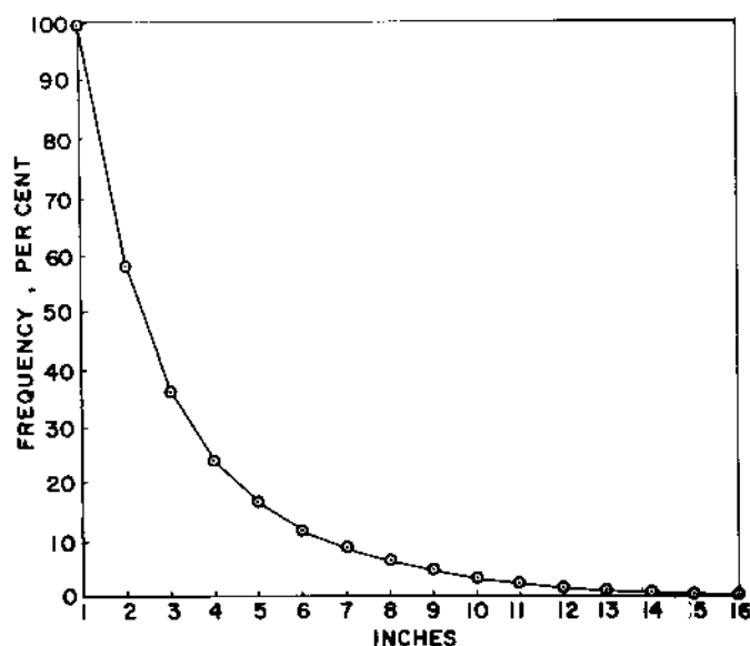
Figure 60. Snowstorm data presented as the frequency of occurrence of total inches of fall per storm in 1931-60, Minneapolis. As an example, a snowstorm will produce a snowfall of 4 inches or more 24 percent of the time.
