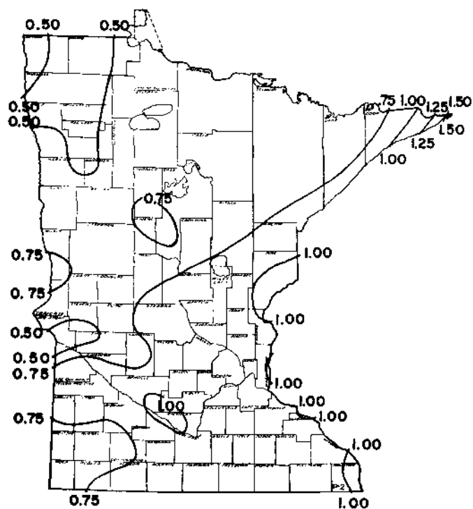
Figure 23. February normal precipitation in inches, Minnesota.
