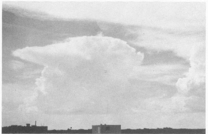
Figure 10. A towering cumulus cloud in the form of domes. It is accompanied by other cumulus at the same base level and dense cirrus at a much higher level. To its right, this same type of cloud is changing to the cumulonimbus (thunder-head) stage. (Collection of the authors)
