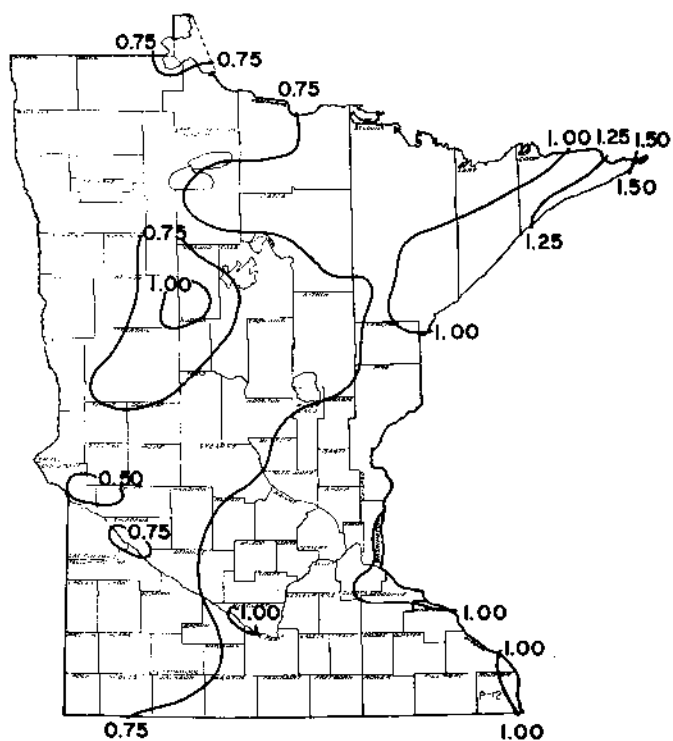
Figure 33. December normal precipitation in inches, Minnesota.
