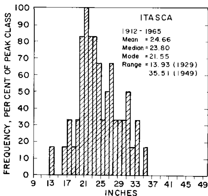
Figure 45. Distribution of annual precipitation in inches in 1912-65, Itasca. Distribution is expressed as a percent of the peak precipitation class.
