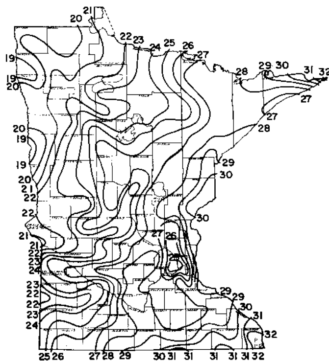
Figure 17. Annual normal precipitation in inches, Minnesota. In general, precipitation increases from the extreme northwest corner to the southeast with a secondary maximum in the northeast and a secondary minimum in the southwest.
