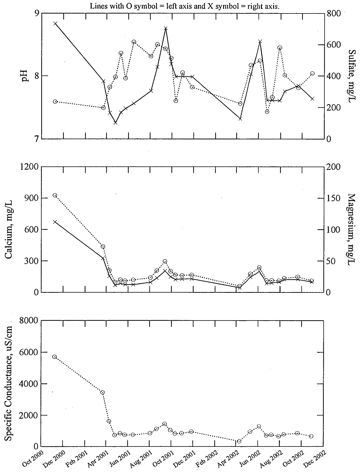
Figure A3.8. Drainage quality vs. time for the limestone addition 1:1 ratio tank 5.
