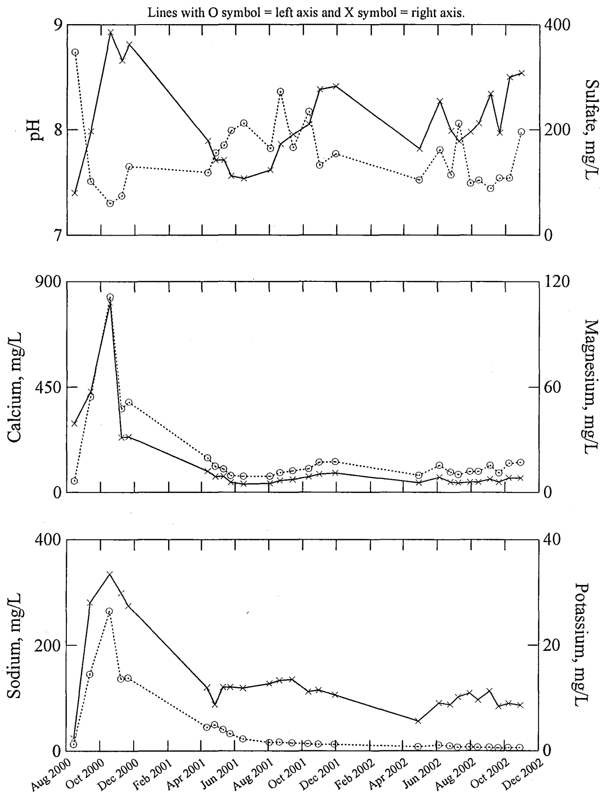
Figure A3.4. Drainage quality vs. time for the 0.67% S prediction field pile 4.
