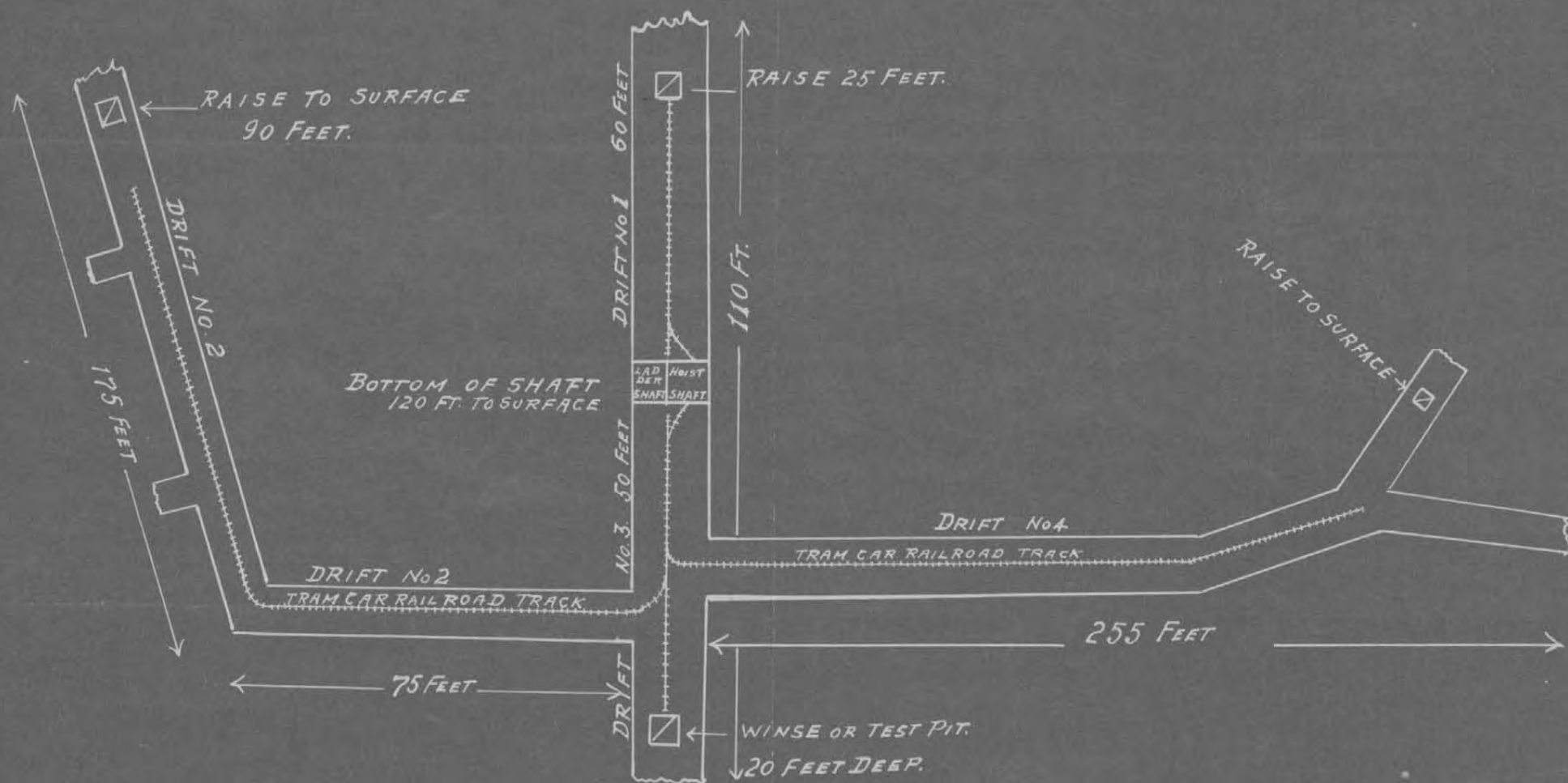
UNDERGROUND DRIFTINGS AJAX MINE. 100 FEET BELOW SURFACE MARCH 20. 1918.
