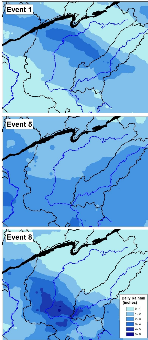
Figure 17. Precipitation distribution (interpolated from National Weather Service radar-based estimates) for Events 1, 5, and 8 (see Figure 7). These events occurred on August 2, 2010, October 27, 2010, and August 2, 2011, respectively. All other events had relatively even precipitation distributions and so are not shown.
