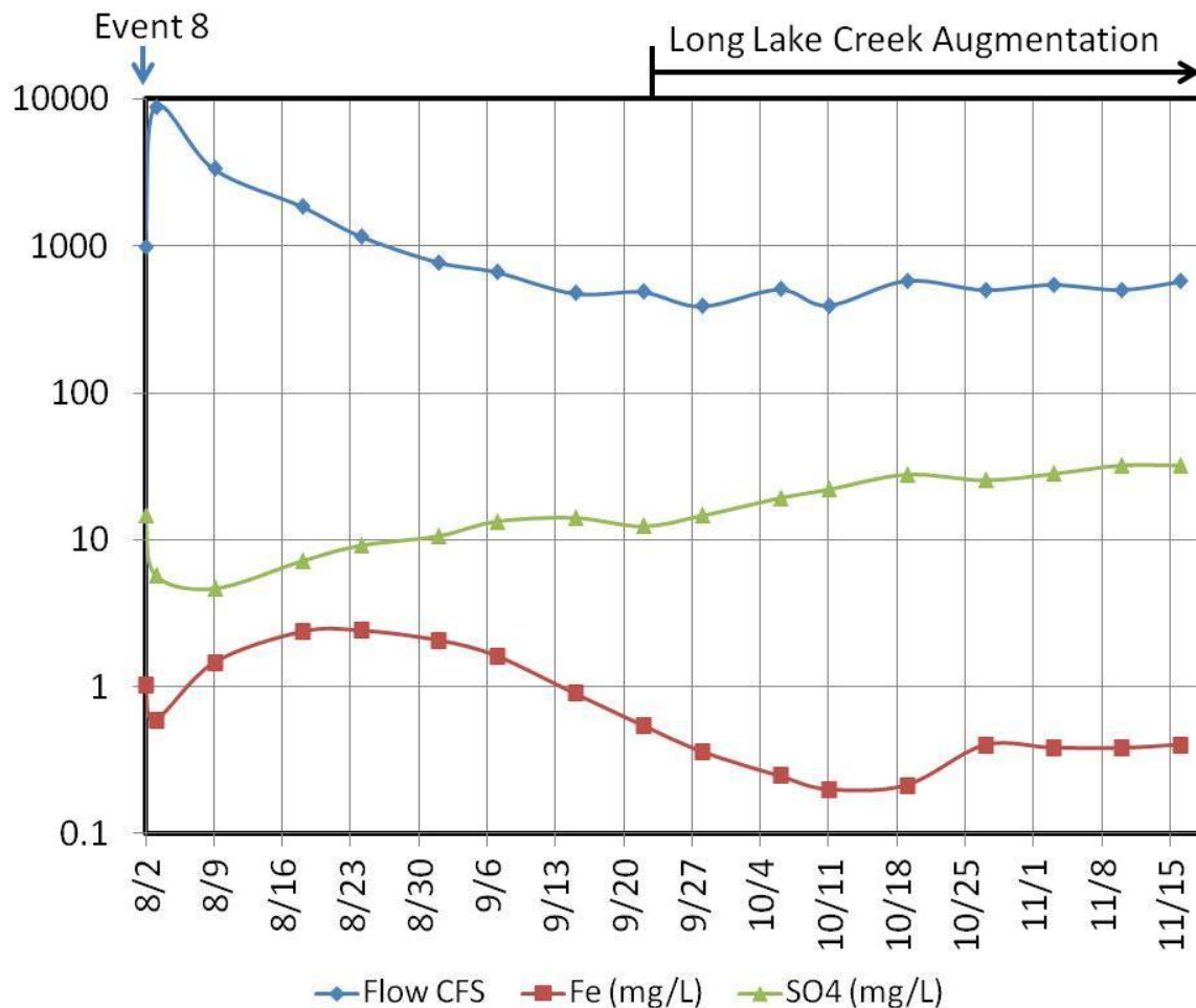
Figure 18. \text{SO}_4^{2-} and Fe concentrations in the St. Louis River following a major rain event over the southern portion of the region (Event 8) that was followed by drought conditions throughout the region. The river was eventually augmented by pumping of mine water through the Long Lake Creek watershed beginning on Sept. 23. This resulted in a further increase in \text{SO}_4^{2-} concentration which precipitated an increase in ionic strength and a decrease in Fe concentrations. The further decrease in Fe is thought to represent deposition of colloidal iron.
