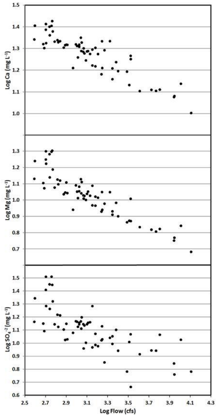
Figure 15. Calcium, magnesium, and SO 4 = concentrations as a function of flow rate for the St. Louis River at Site 001 and Scanlon Dam. Under low flow conditions, the St. Louis River has a disproportionate amount of water containing these components, which are elevated in streams that originate in the mining region. Similar negatively sloping trends are observed for chloride, fluoride, strontium, and sodium (provided in Appendix A3).
