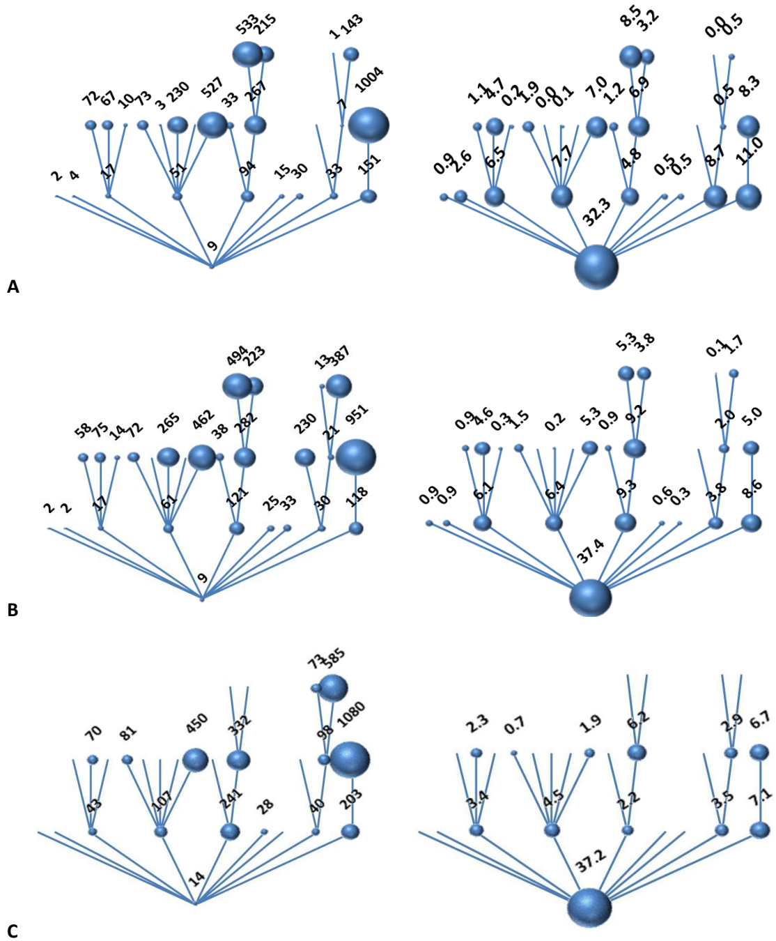
Figure 4. \text{SO}_4^{=} concentrations ( \text{mg L}^{-1} , on left) and loads (metric tons/day, on right) determined in this study for August (A), September (B), and March (C).
