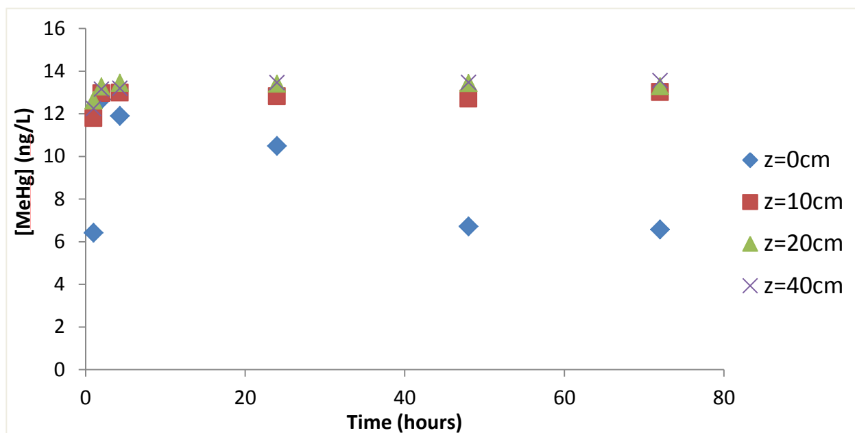
Figure 2. Photodemethylation of \text{MeHg}^+ in St. Louis River water at various depths. Samples were irradiated in the field in sealed 10 mL quartz tubes.
