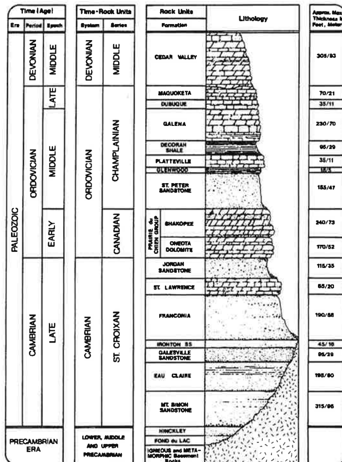
Minnesota's Sedimentary Rock Column (after Weber and Austin, 1972, as reported in Ojakangas and Matsch, 1982).
