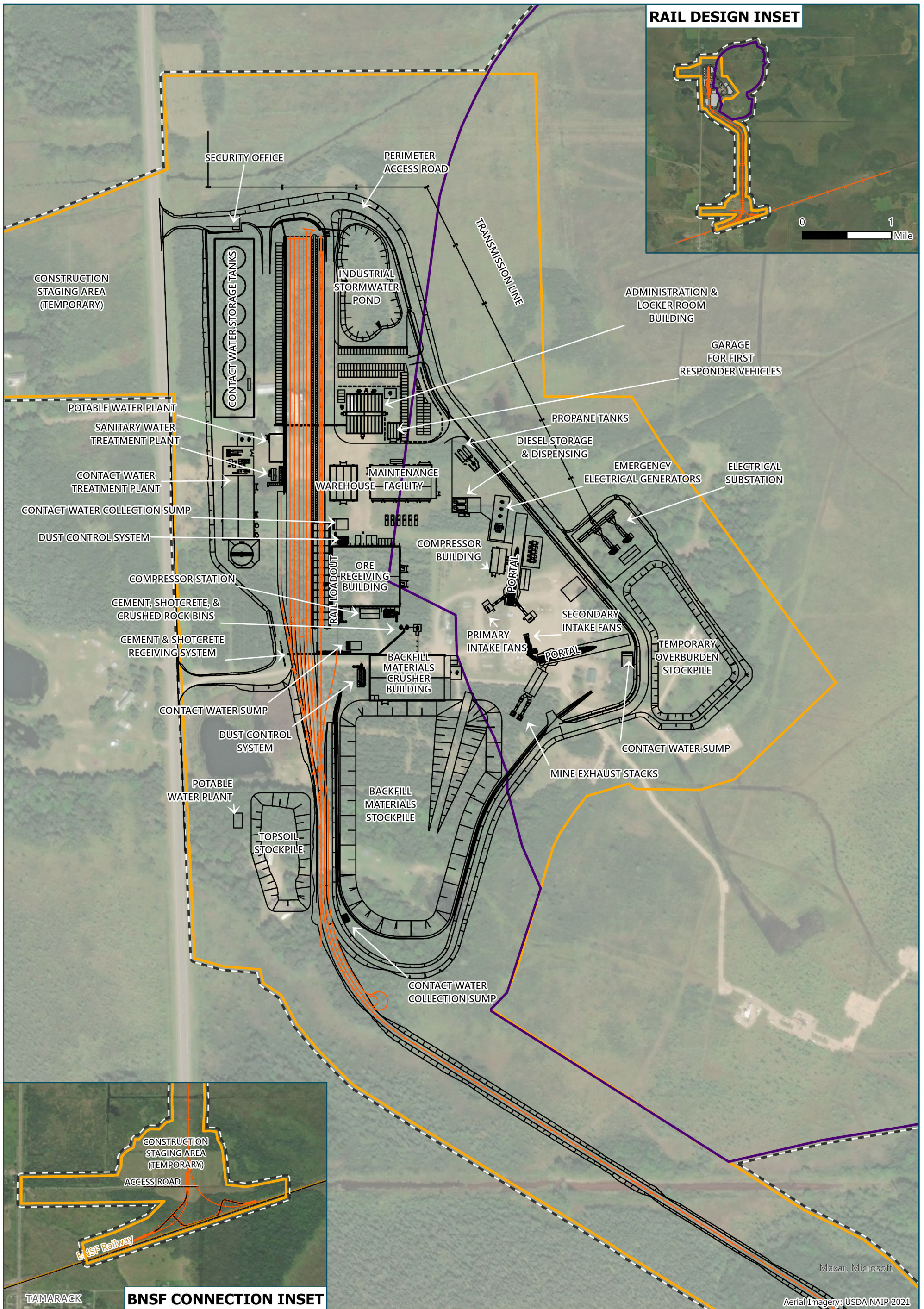
SITE LAYOUT Tamarack Mining Project Figure 3 Environmental Assessment Worksheet
