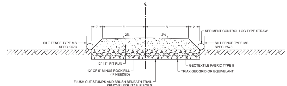
TYPICAL C WETLAND CROSSING ATV AND SNOWMOBILE (20' OVERALL WIDTH)
