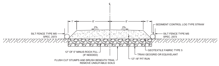
TYPICAL A WETLAND CROSSING ATV AND SNOWMOBILE (14' OVERALL WIDTH)
