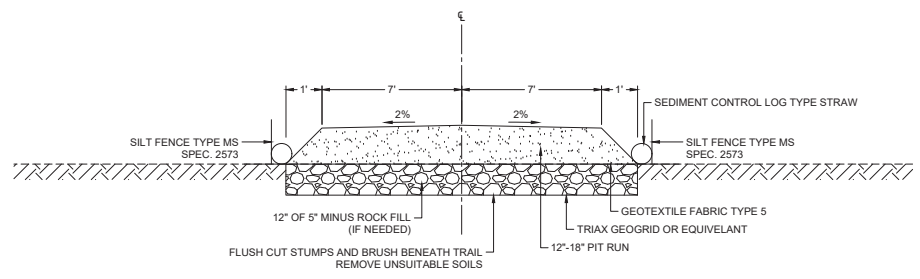
TYPICAL D WETLAND CROSSING ATV AND SNOWMOBILE (16' OVERALL WIDTH)
