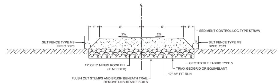
TYPICAL B WETLAND CROSSING ATV ONLY (12' OVERALL WIDTH)
