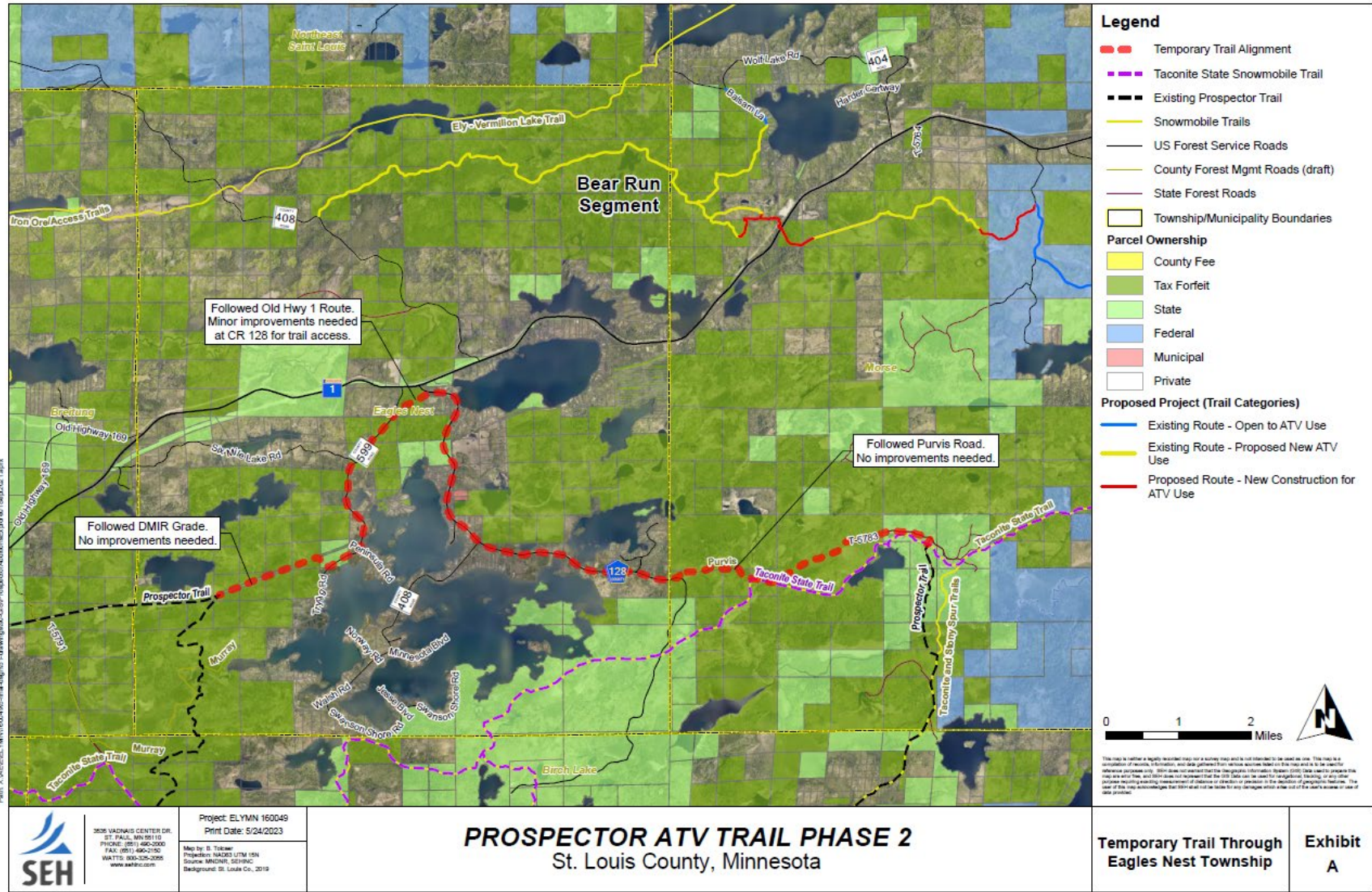
Figure 1. The image shows the Prospector ATV trail temporary trail alignment (in red dashed lines) near Eagles Nest Township, along with land use types, and the current (black dashed lines) and proposed project trails (in yellow and red lines).
