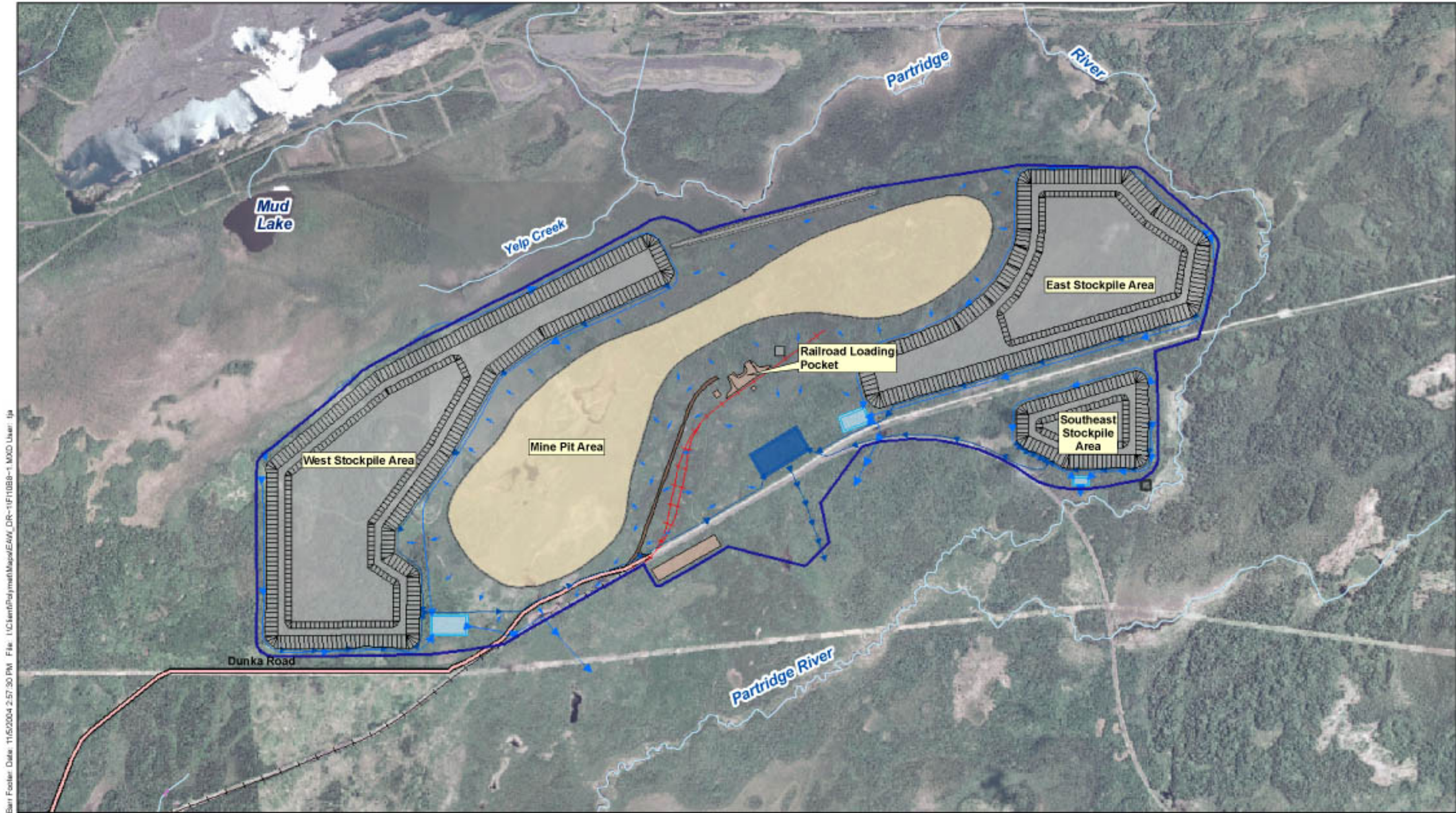
Figure 5-3 MINE AND STOCKPILES SITE PLAN
