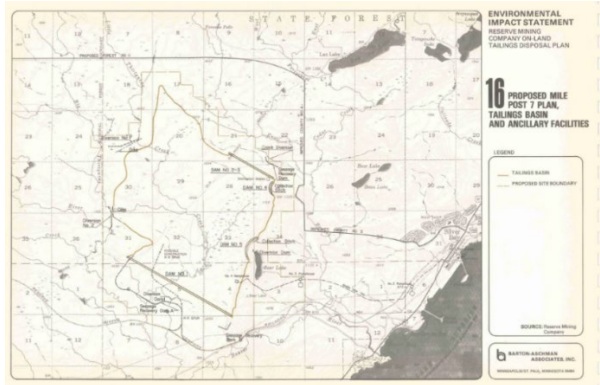
Figure 16: Proposed Mile Post 7 Plan, Tailings Basin, and Ancillary Facilities
