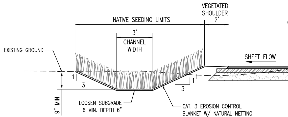
TYPICAL INFILTRATION BASIN
