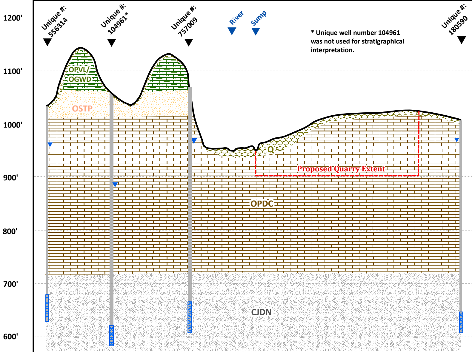
Figure 11: Well Locations Cross-Section A - A'
