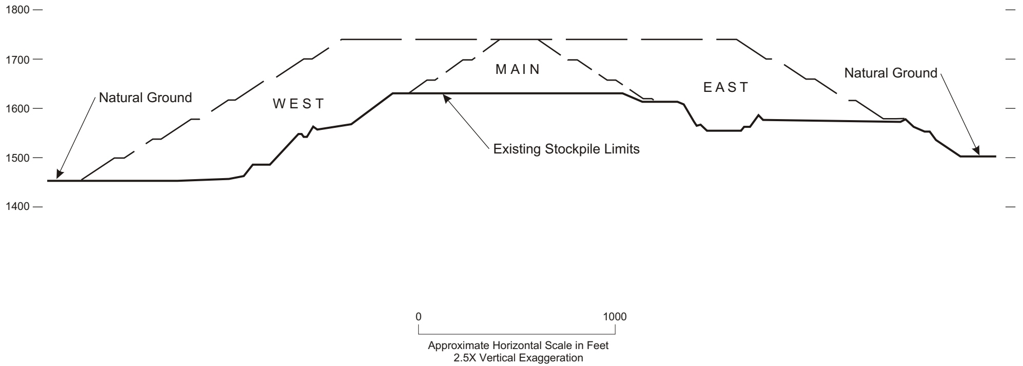
Figure 6-2 CONCEPTUAL CROSS SECTION AREA 2WX STOCKPILE Mesabi Nugget Hoyt Lakes, Minnesota
