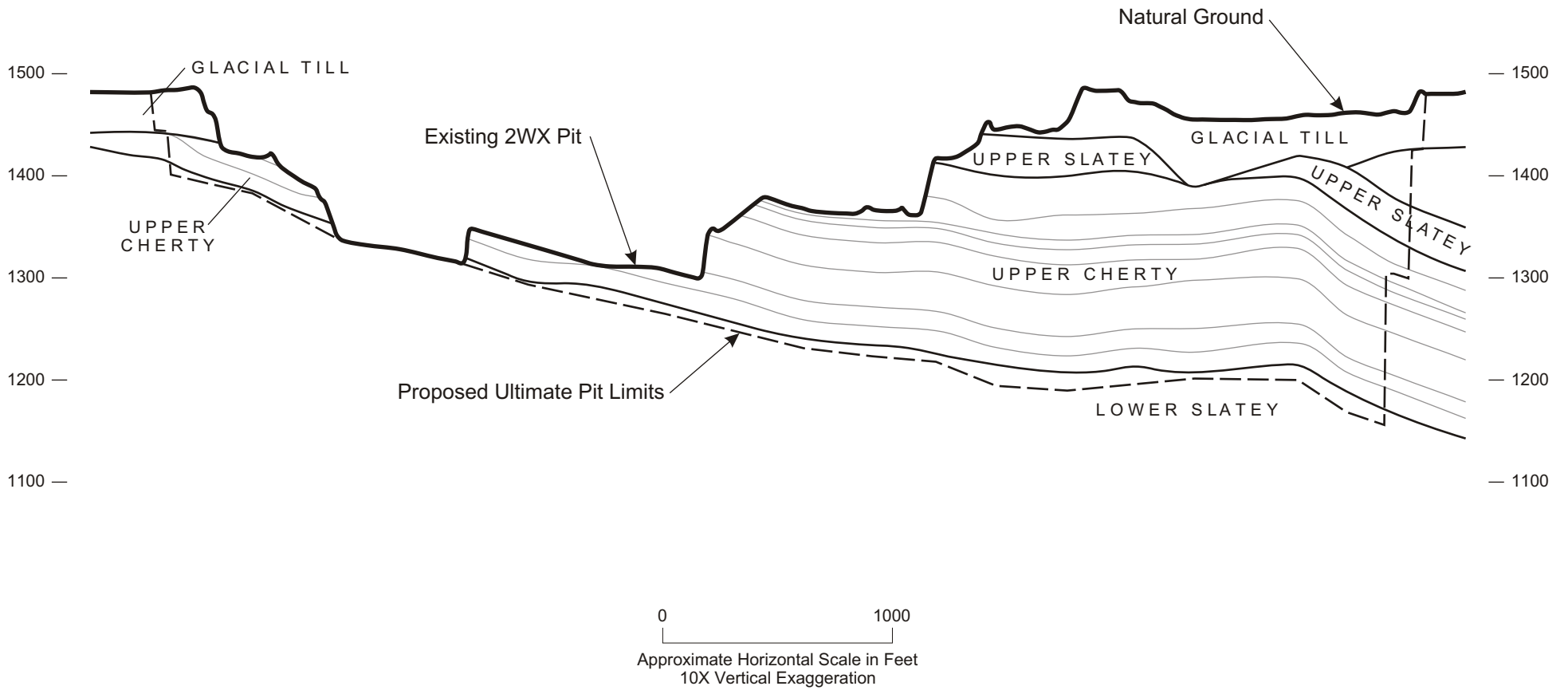
Figure 6-1 CONCEPTUAL CROSS SECTION AREA 2WX PIT Mesabi Nugget Hoyt Lakes, Minnesota
