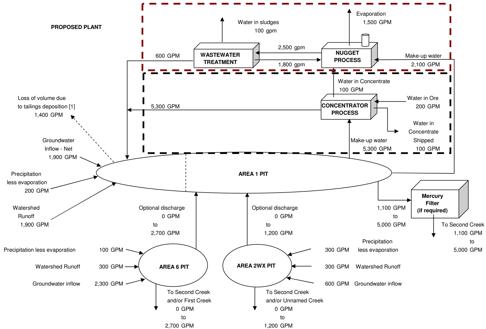
Figure 13-1 Preliminary Project Water Balance
