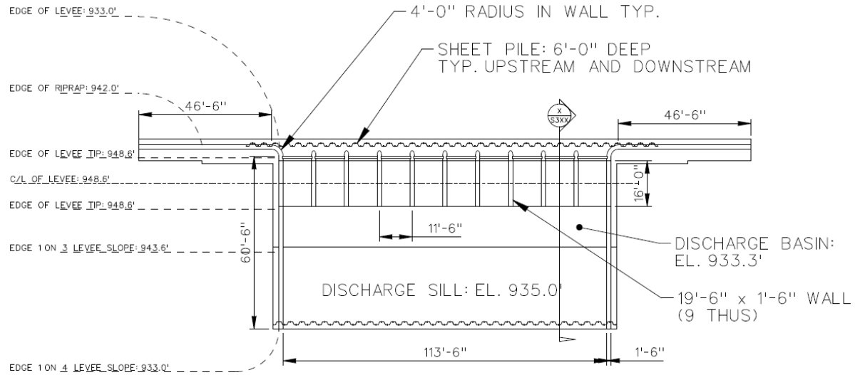
PLAN VIEW - DRAWDOWN STRUCTURE
