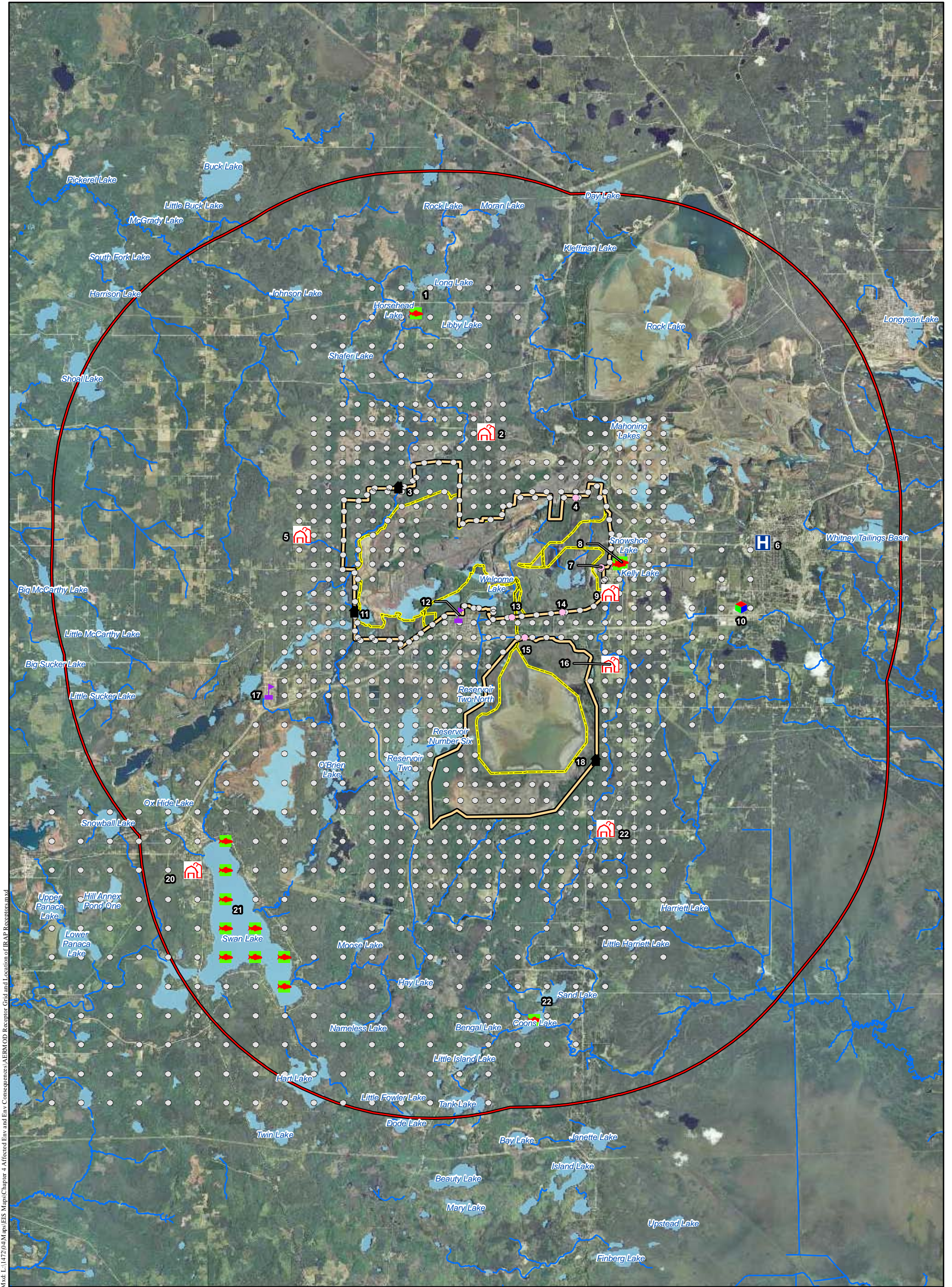
Figure 4.9.8.1 AERMOD Receptor Grid and Location of IRAP Receptors U.S. Steel Keetac Keewatin, MN
