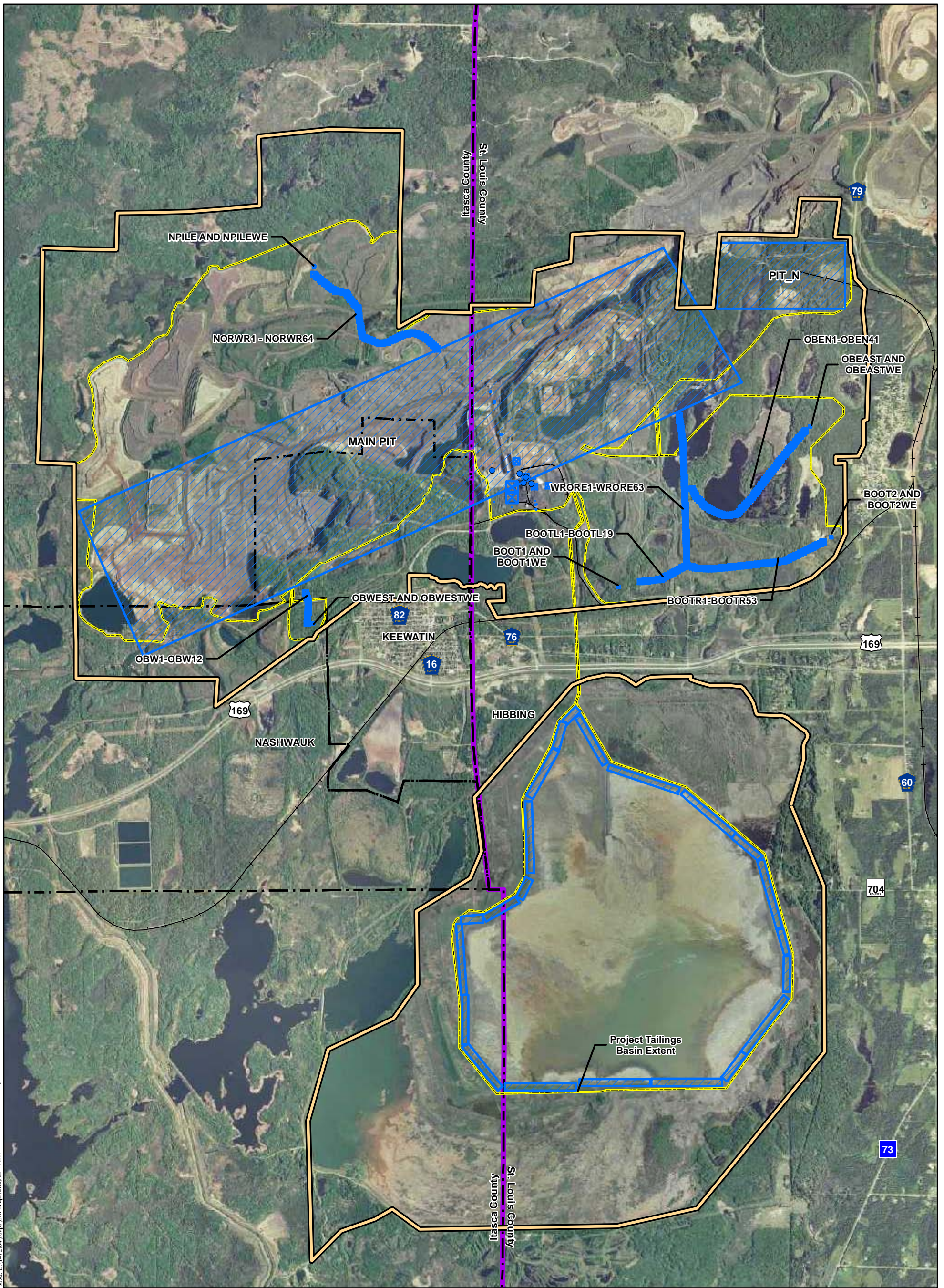
Figure 4.9.6.4 Proposed Project Mine Plan NAAQS Sources U.S. Steel Keetac Keewatin, MN
