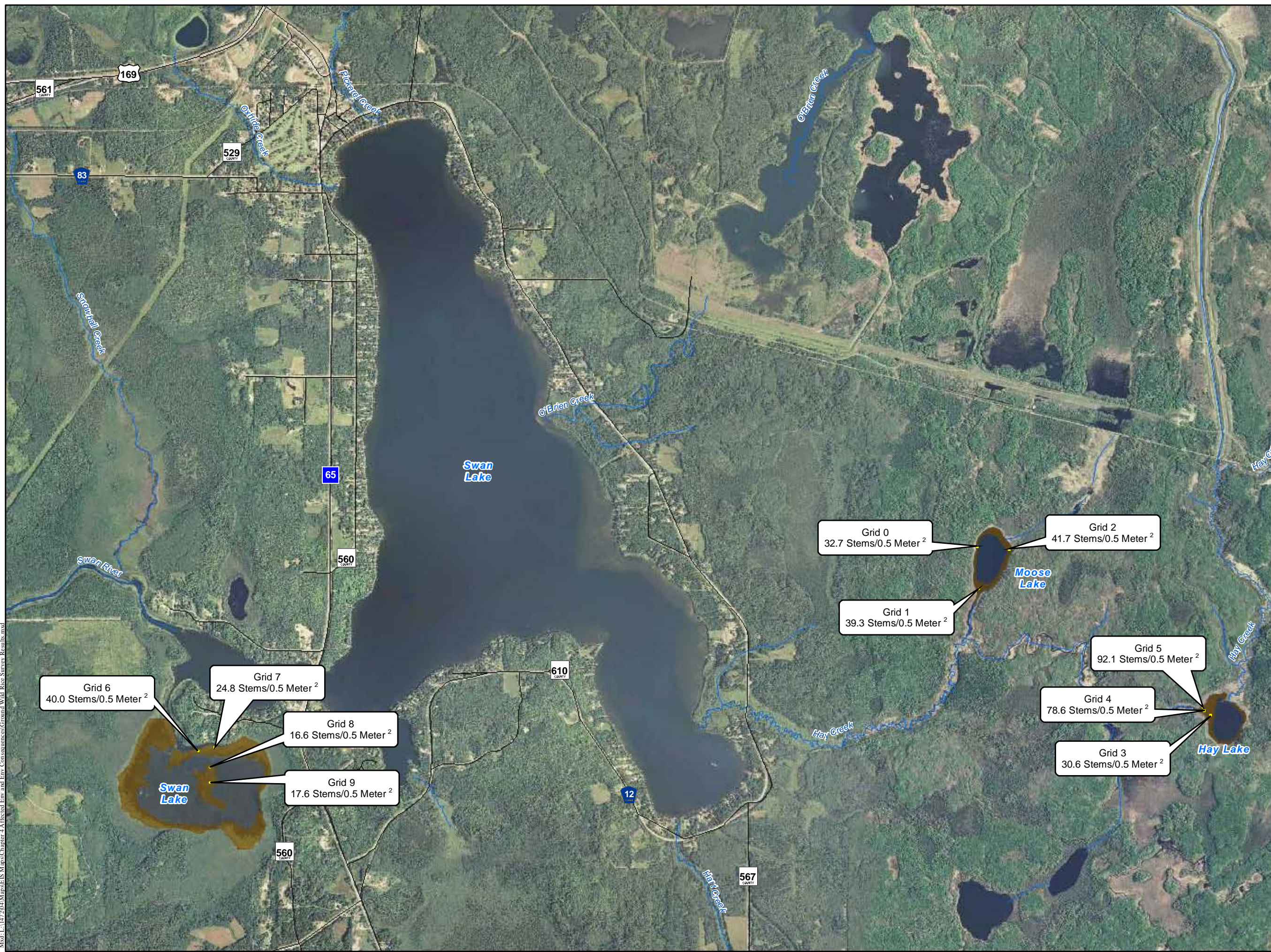
Figure 4.7.2 Wild Rice Survey Results for Swan Lake SW Bay, Moose and Hay Lakes U.S. Steel Keetac Keewatin, MN
