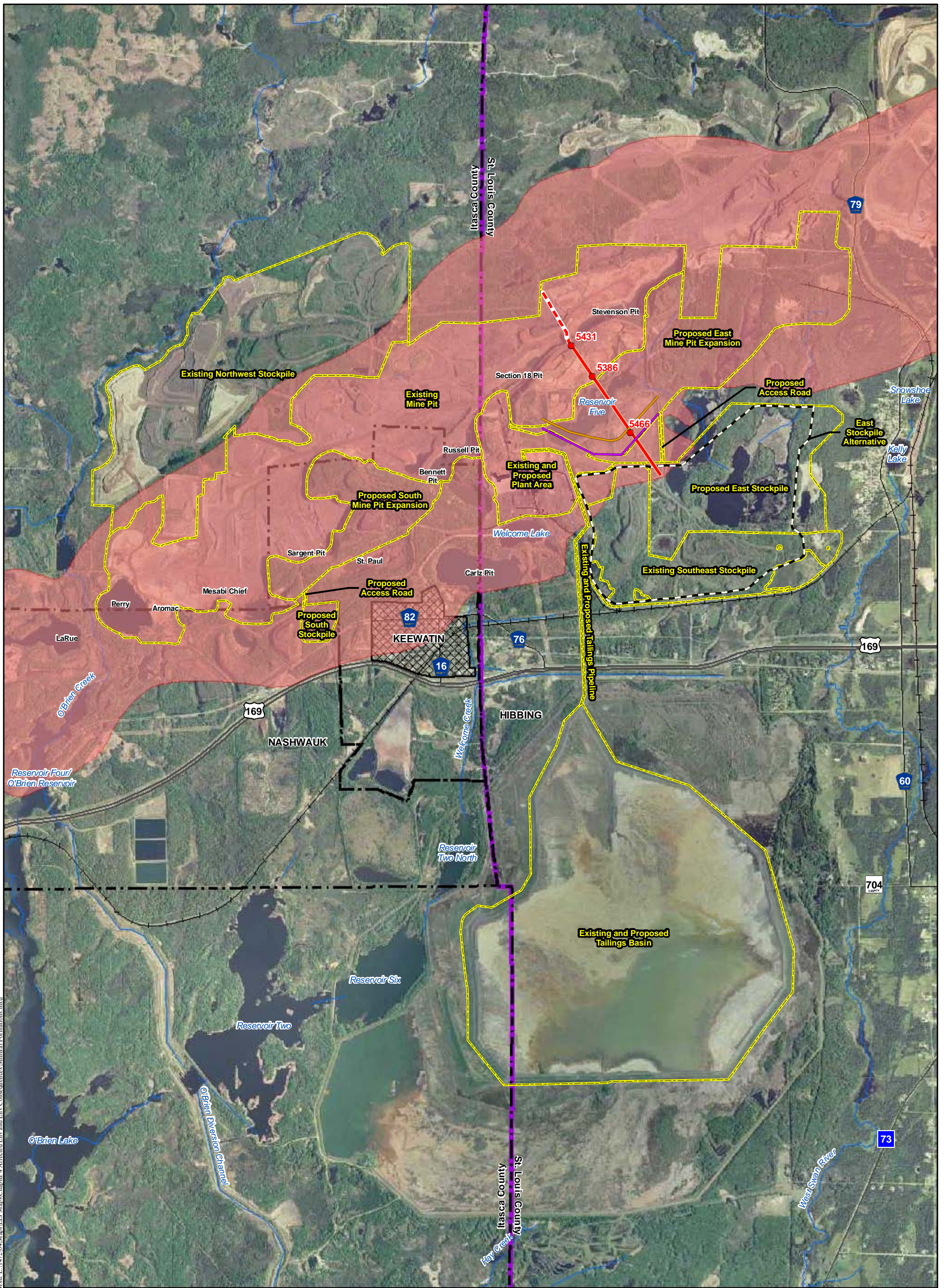
Figure 4.23.1 Mineral Formations U.S. Steel Keetac Keewatin, MN
