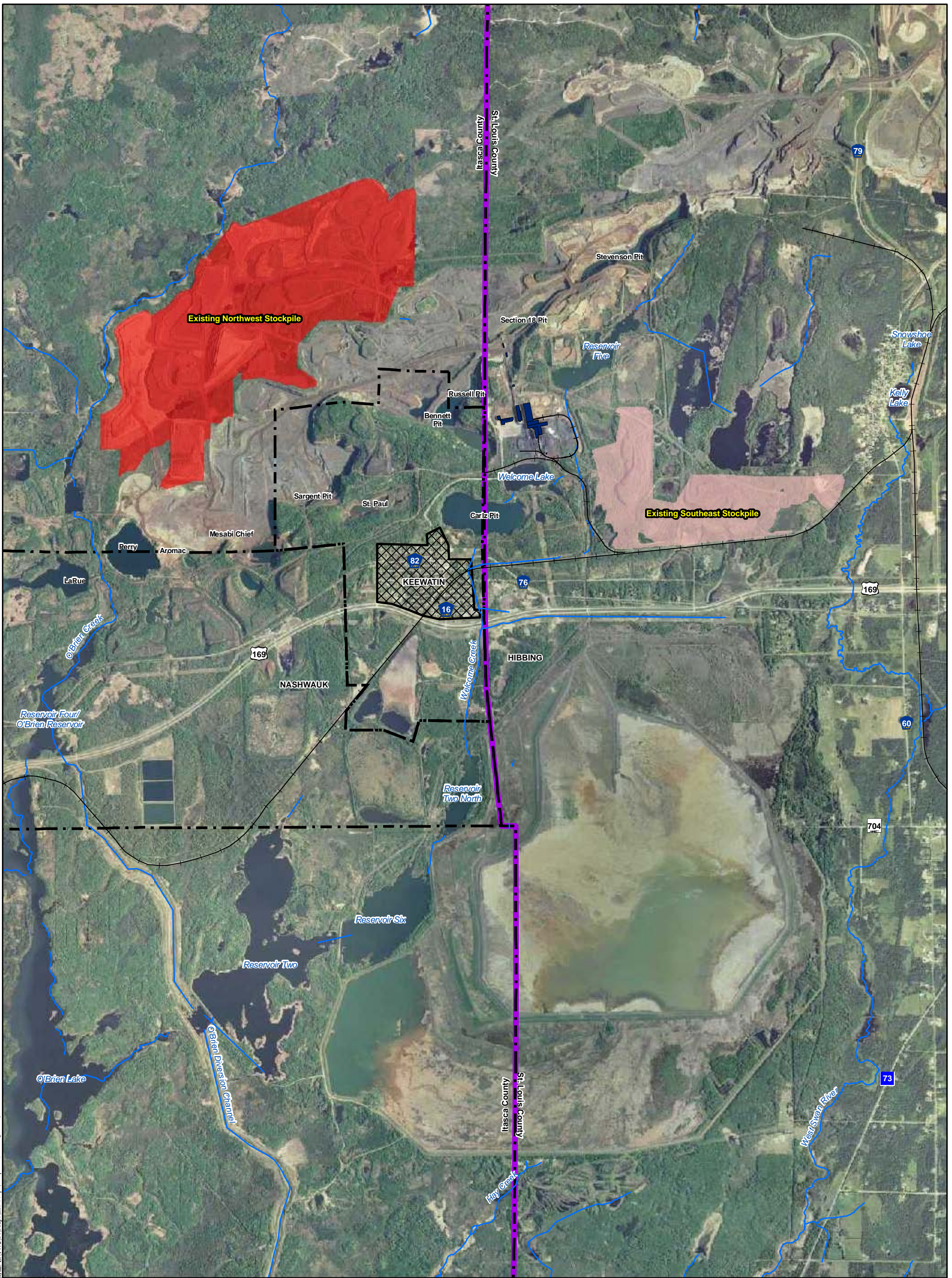
Figure 3.2.2 Existing Out of Pit Stockpiles U.S. Steel Keetac Keewatin, MN
