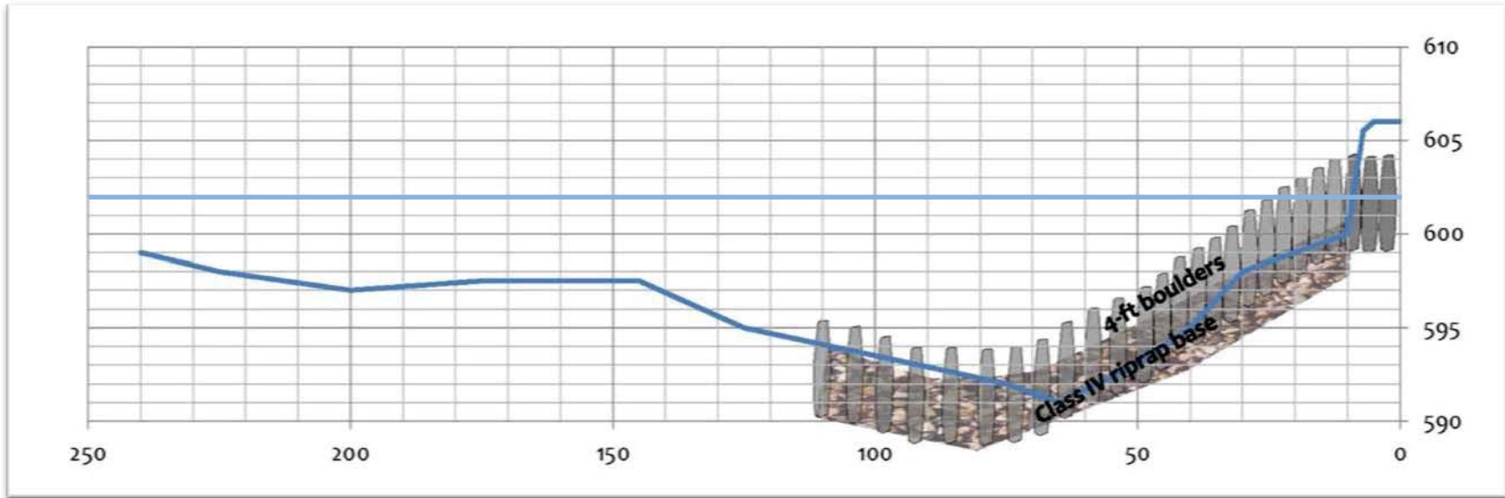
Figure 8: J-hook cross sections at 6+00. Cross sections align at 30° upstream angle. Average low water elevation is 602 feet above mean sea level.
