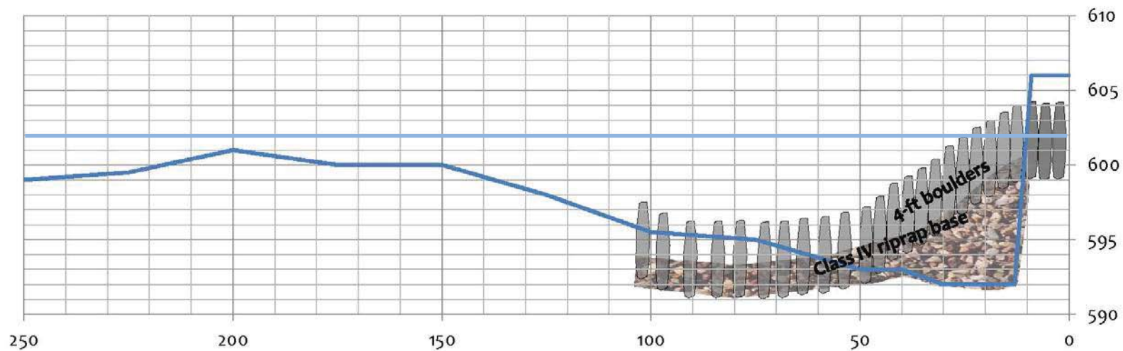
Figure 7: J-hook cross sections at 2+50. Cross sections align at 30° upstream angle. Average low water elevation is 602 feet above mean sea level.
