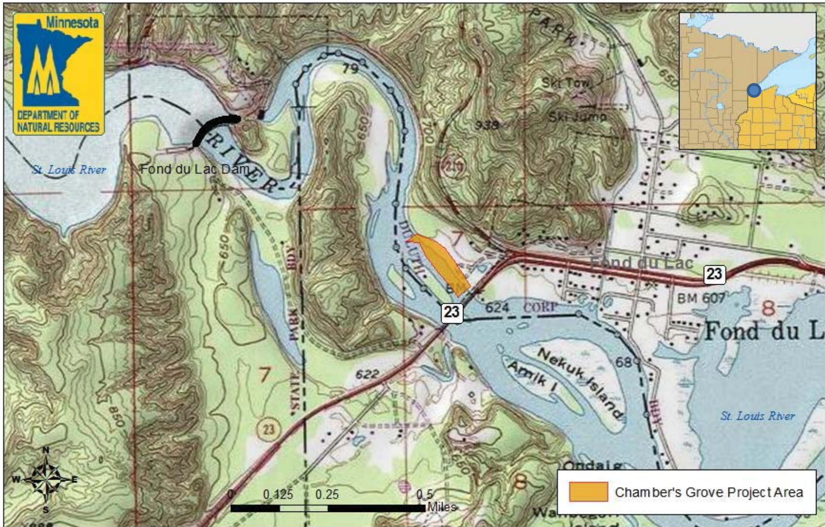
Figure 2: Topographic map of Chambers' Grove Aquatic Habitat Restoration Project near Fond du Lac, MN. Project area located approximately 1.4 miles downstream of the Fond du Lac dam on the St. Louis River near Minnesota State Highway 23.
