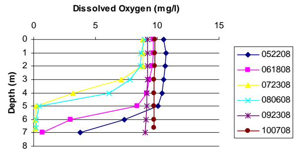
Carrie Lake 2008 Dissolved Oxygen Profiles
