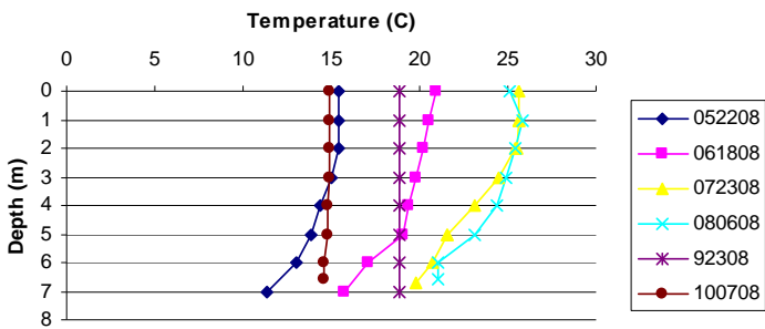
Carrie Lake 2008 Temperature Profiles
