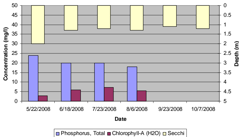
2008 Carrie Water Chemistry
