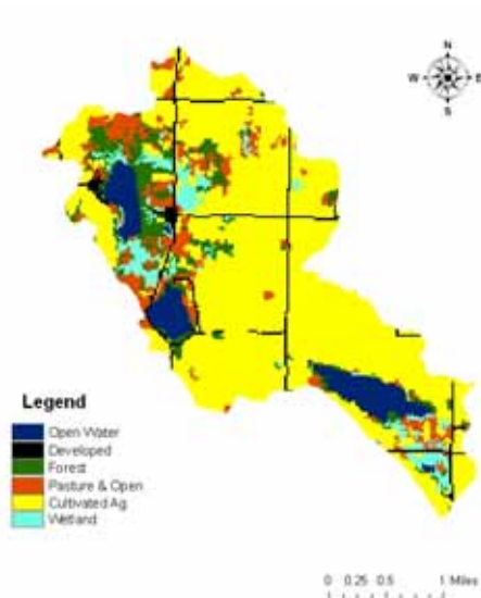
Figure 2. Lake Carrie Watershed land use
