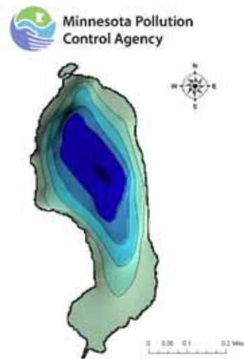
DNR Ecological Services & Fisheries Divisions 2002 Lake Bathymetric DEM Shaded Relief Image
