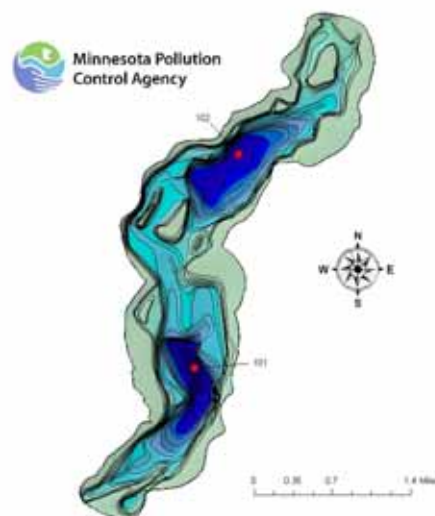
DNR Ecological Services & Fisheries Division 2002 Lake Bathymetric DEM Shaded Relief Image
