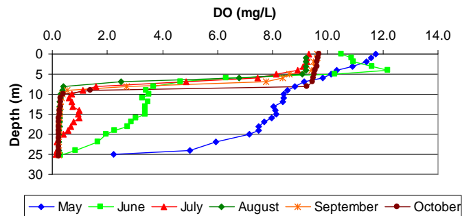
Elk lake 2008 Dissolved Oxygen Profiles
