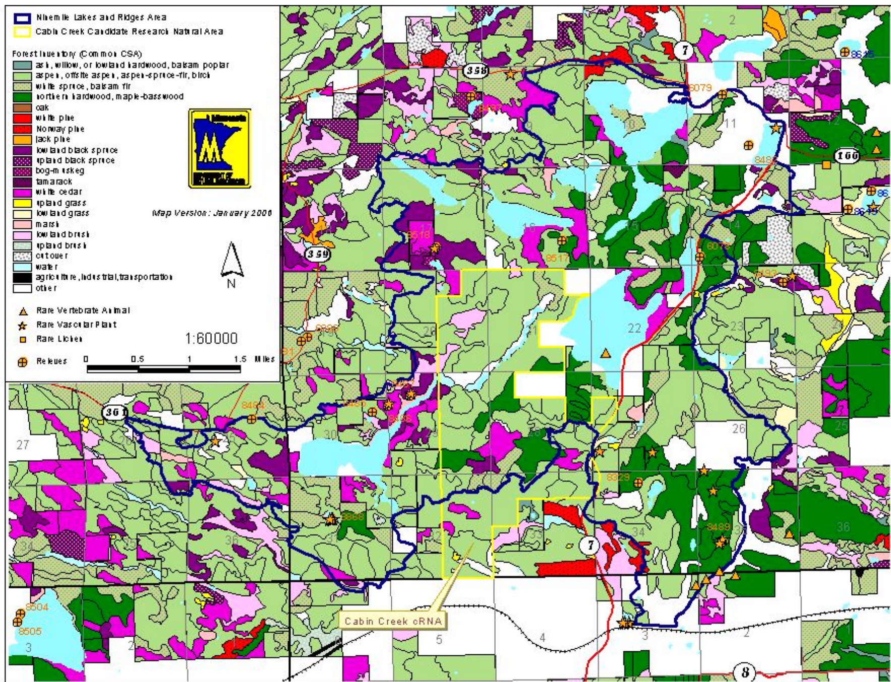
Figure 6. Forest Inventory Cover Types (Common CSA) for Ninemile Lakes and Ridges area.
