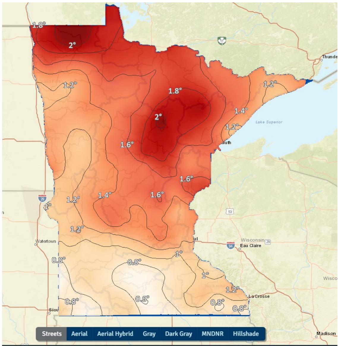
Figure 6.11. Annual average temperatures (1991-2020) deviation when compared to historical average (1895-2020) (DNR Geospatial Commons 2024).
