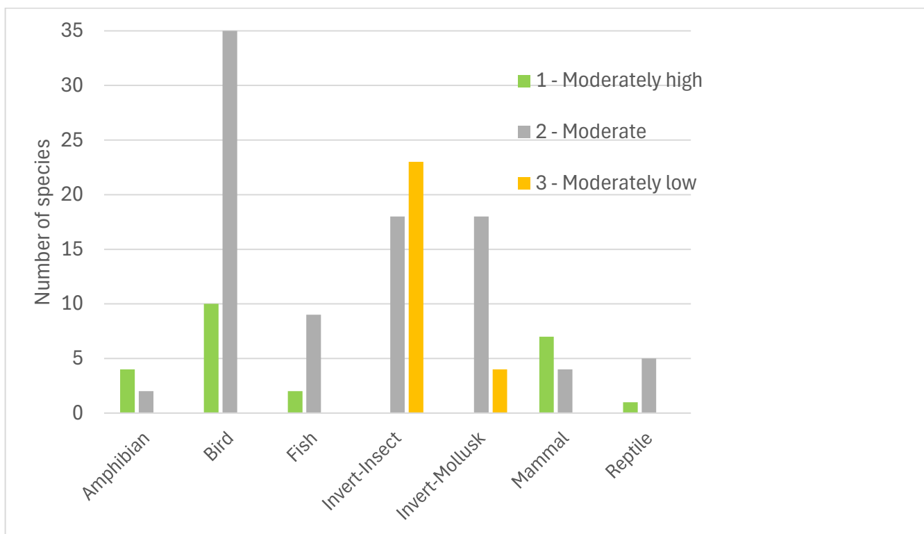
Figure 6.14. Graph indicating the overall adaptive capacity assessment scores for Minnesota SGCN evaluated in the Michigan-led adaptive capacity assessment study (Earl et al., 2024).
