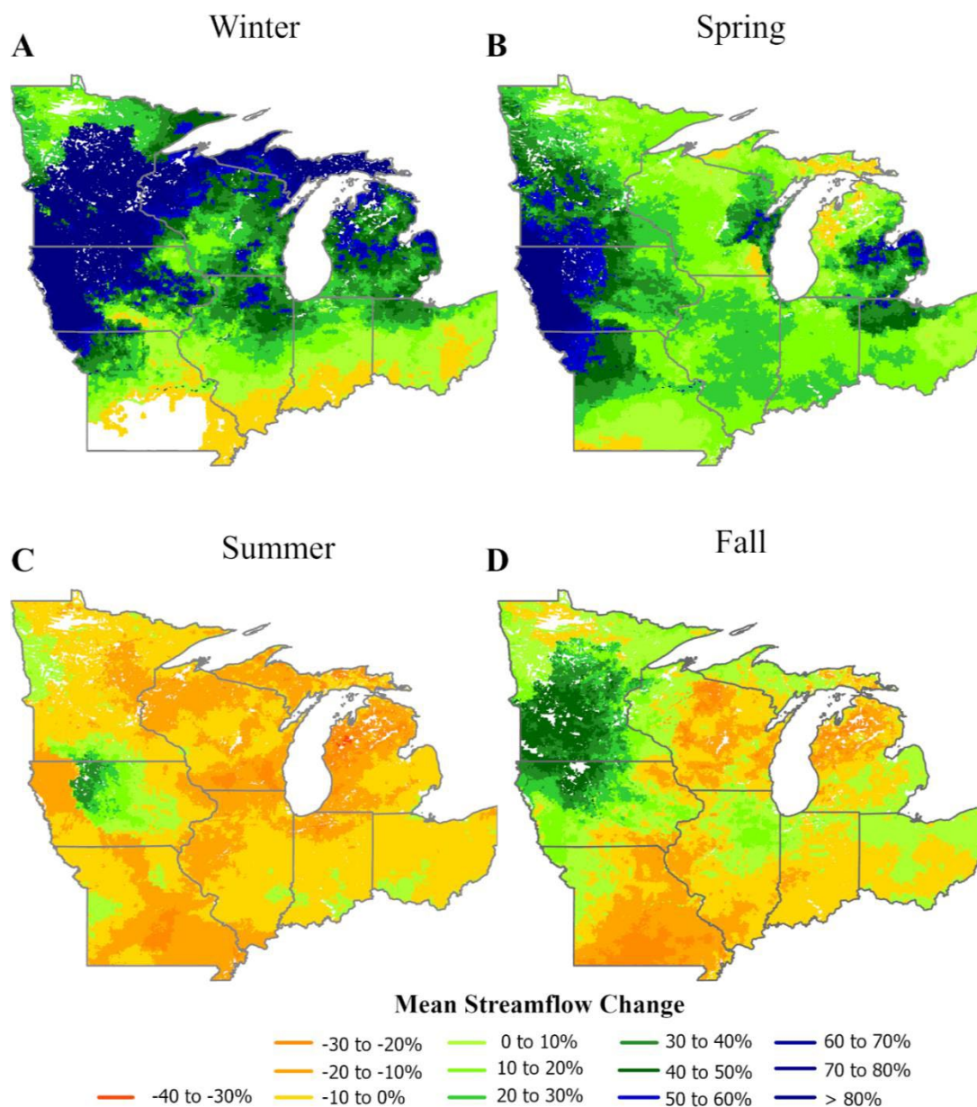
Figure 3.14. (from Ratcliffe et al. 2025). Projected changes in mean streamflow in the Midwest. Projections use gridded simulations of daily runoff based on CMIP5 climate models under the high-emissions (RCP 8.5) scenario. Values show the percent change in mean daily streamflow (cubic feet per second) for each season (winter, December–February; spring, March–May; summer, June–August; fall, September–November) at the end of the century (2070–2099) compared to historical data (1977–2006). Data and metric definitions are provided by the U.S. Stream Flow Metric Dataset (Authors (in review); U.S. Department of the Interior, Bureau of Reclamation, 2014; USDA Forest Service Office of Sustainability and Climate, 2022; Wenger and others, 2010).
