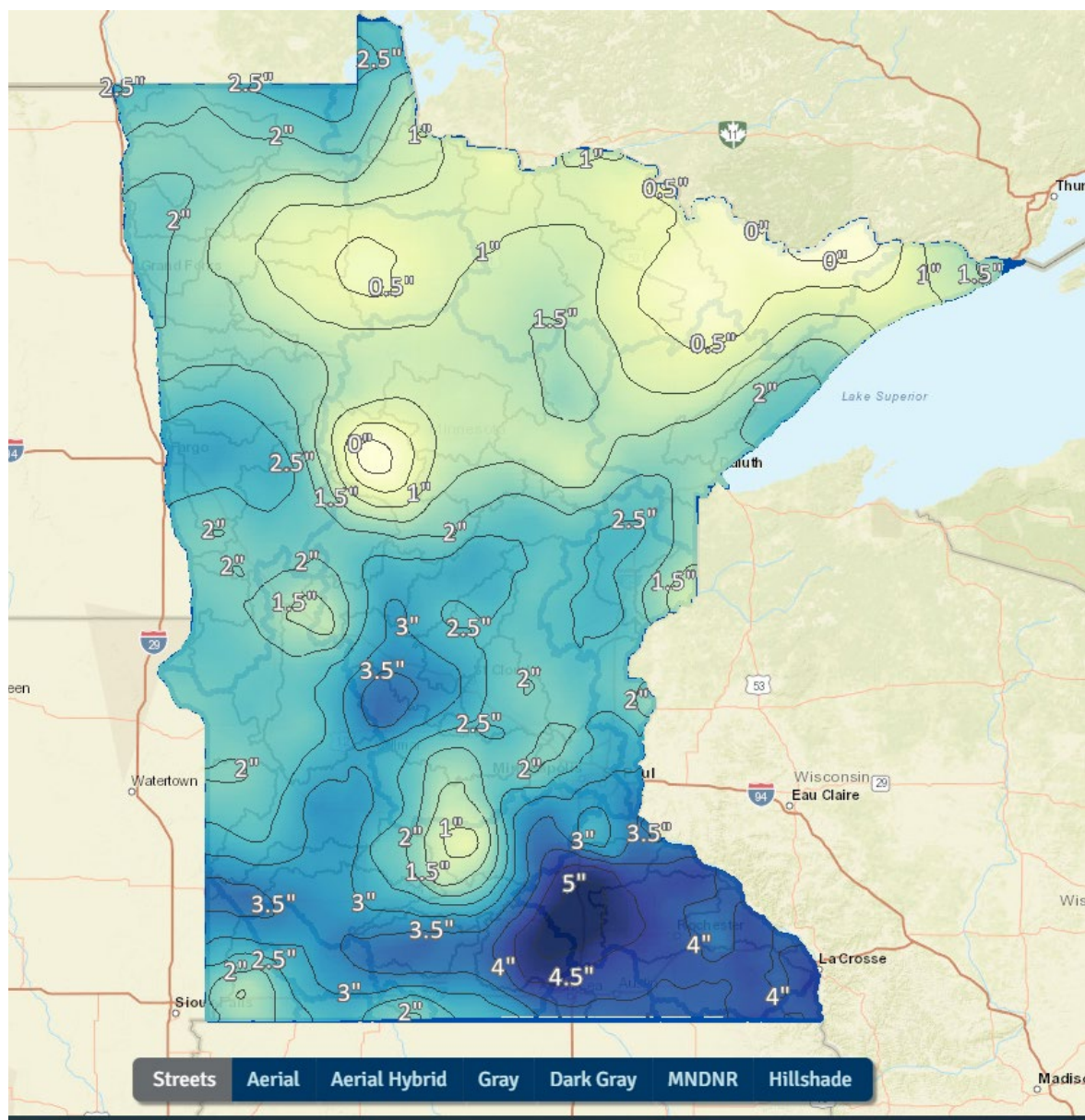
Figure 6.12. Annual average precipitation (1991-2020) deviation when compared to historical average (1895-2020) (DNR Geospatial Commons 2024).
