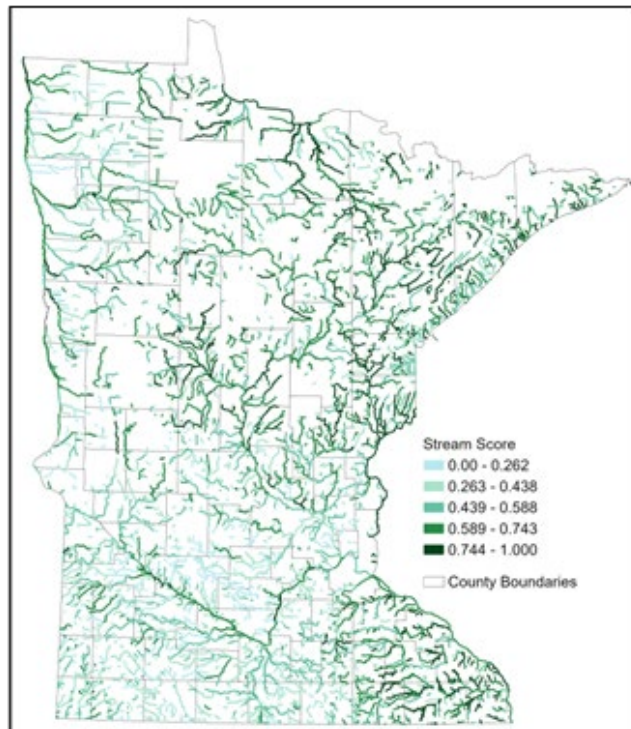
Figure 6.6. Stream score from the maximum fish or invertebrate IBI value by stream segment (WID) normalized to a range between 0 and 1.
