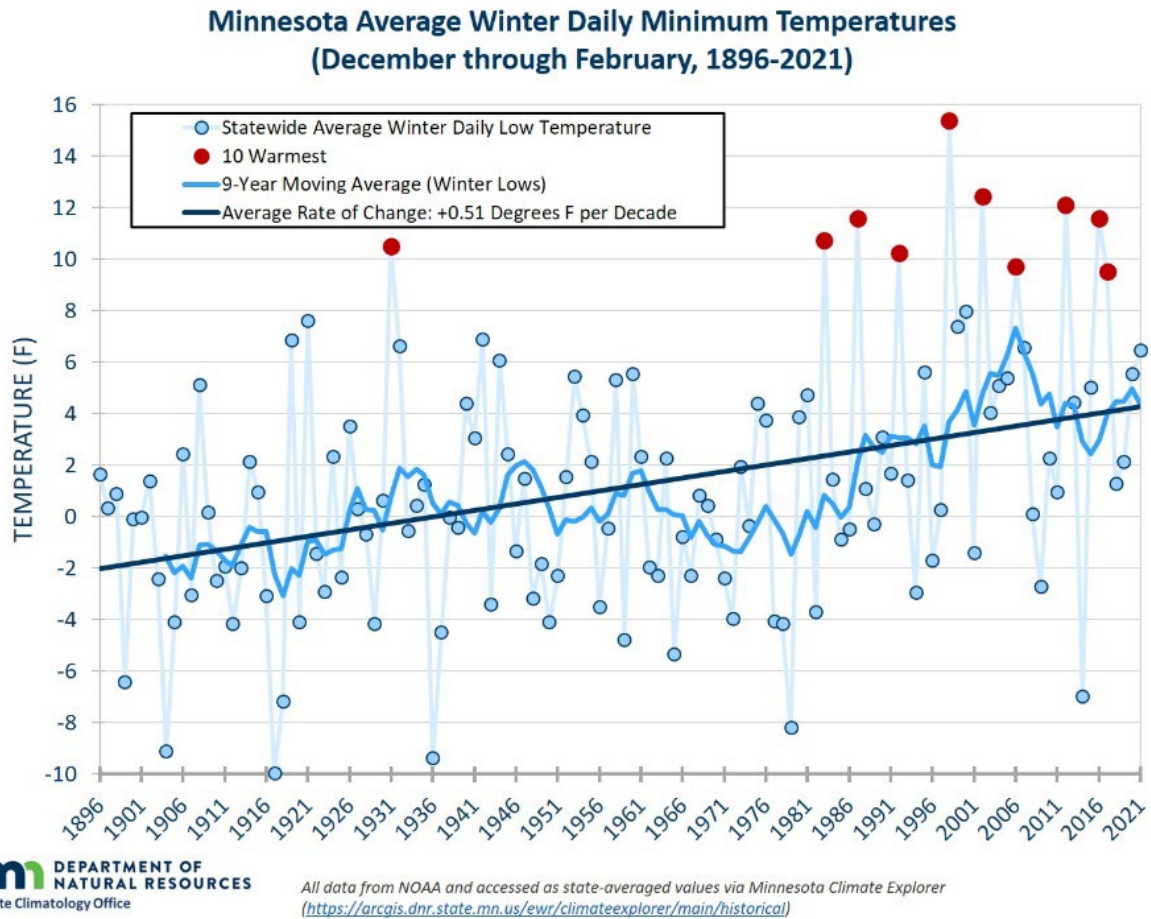
Figure 6.10. Chart depicting Minnesota Average Winter Daily Minimum Temperatures (December through February 1896 – 2021) by the DNRState Climatology Office based on data from the Minnesota Climate Explorer.
