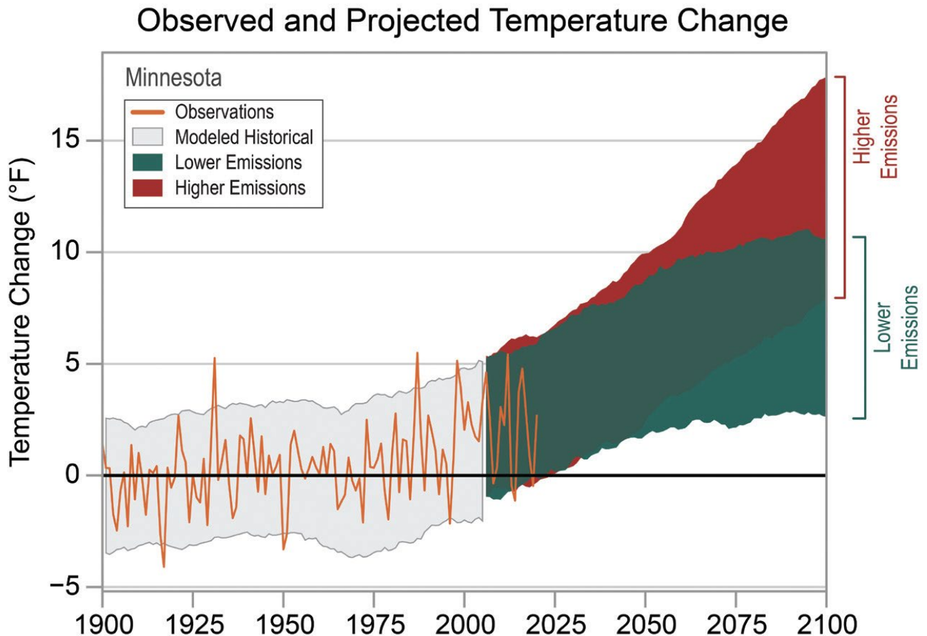
Figure 6.13. Observed and projected temperature changes in Minnesota under “lower” (teal) and “higher” (red) emissions scenarios out to 2100 compared to historical temperature observations (orange). Figure from: Runkle, J., K.E. Kunkel, R. Frankson, D.R. Easterling, S.M. Champion, 2022: Minnesota State Climate Summary 2022. NOAA Technical Report NESDIS 150-MN. NOAA/NESDIS, Silver Spring, MD, 4 pp.
