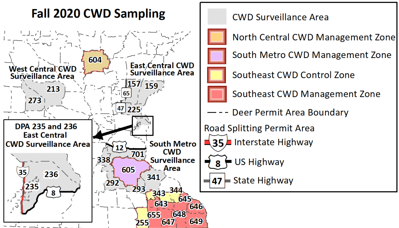
Figure 2. Areas for chronic wasting disease surveillance of hunter-harvested deer planned for fall 2020 in Minnesota.
