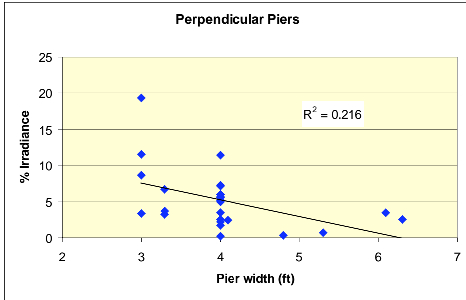
Figure 4. Relation between amount of light under a pier versus pier width.
