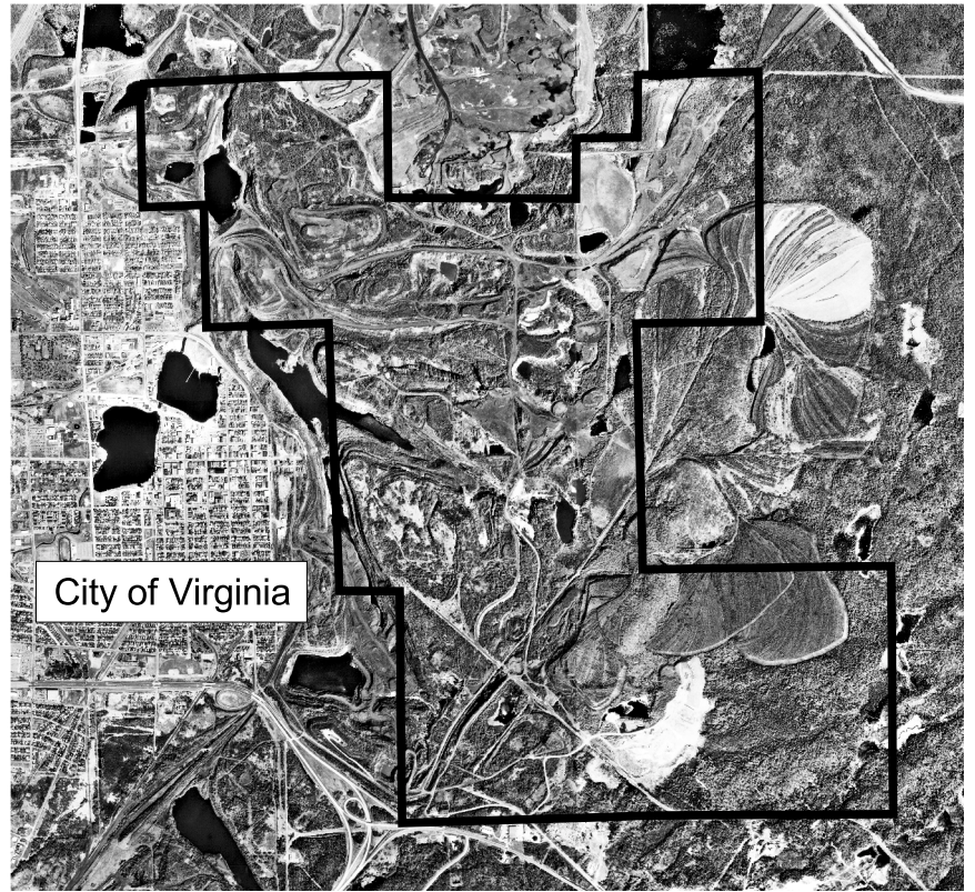
Figure 2. Virginia and Calumet Study Areas
