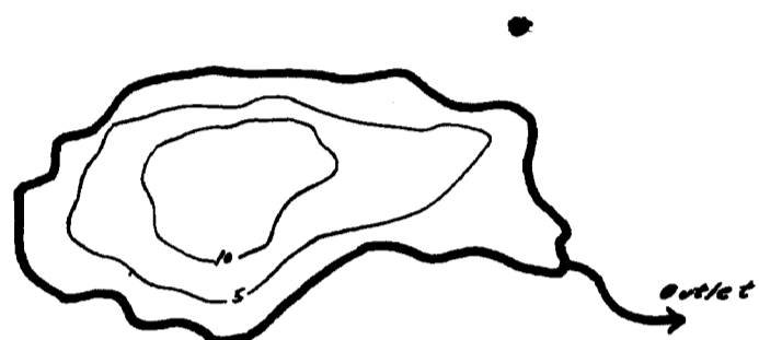
Contour Map Contour Interval - 5ft.
