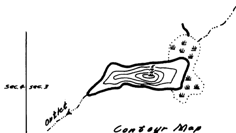
Contour Map Interval - 5ft.
