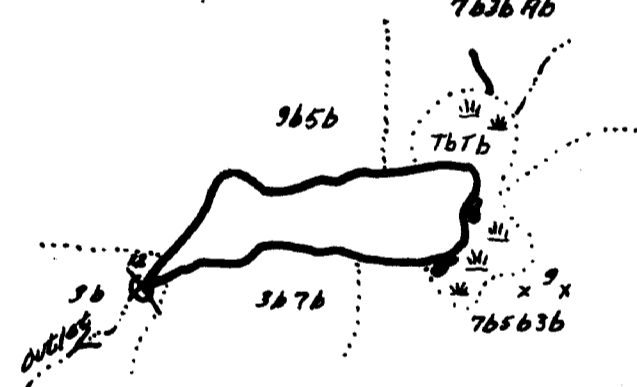
Shoreline, Cover Type Map
