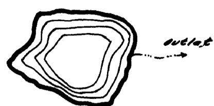
Contour Map Interval - 5ft.
