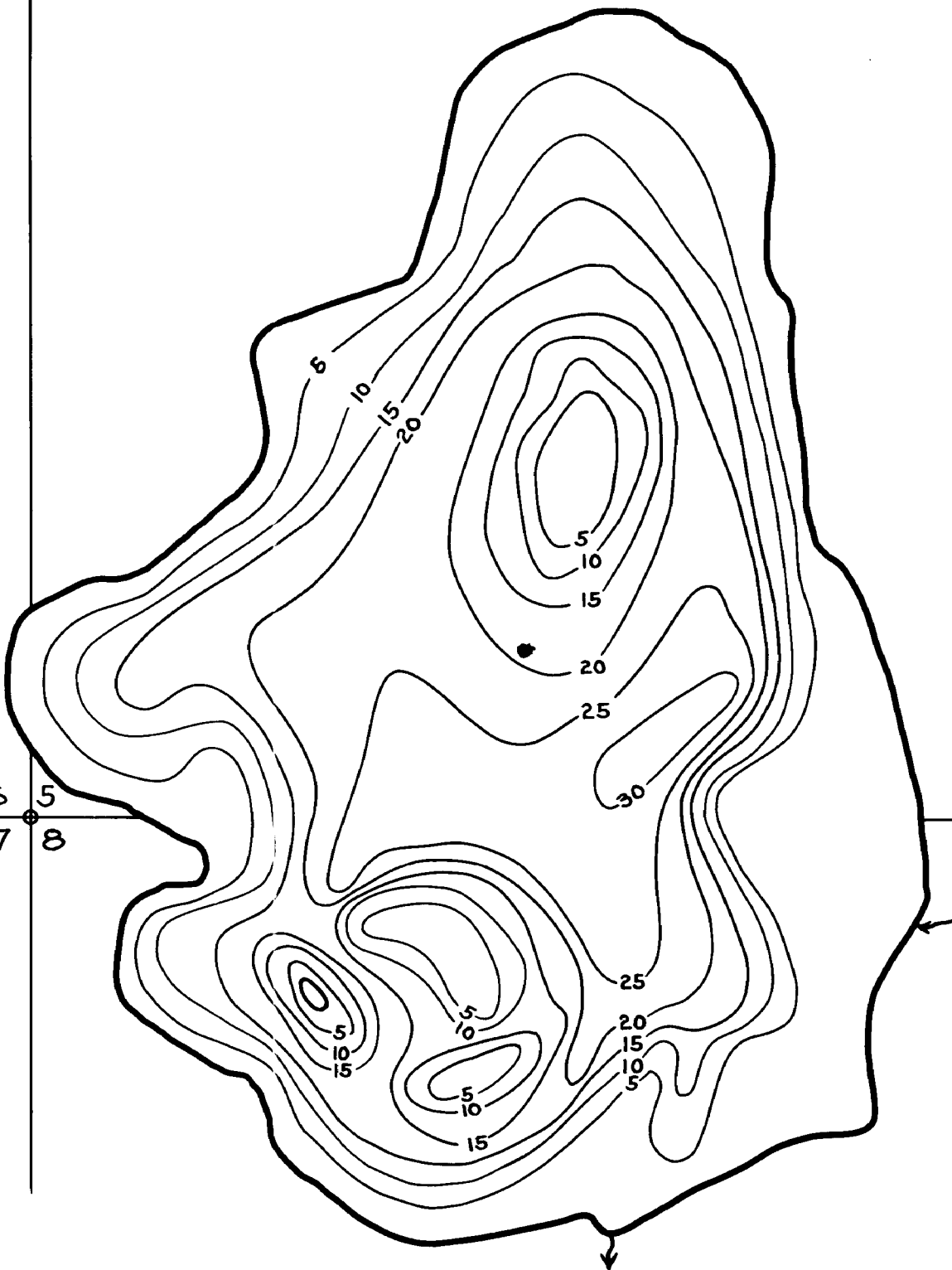
Contour Map Contour Interval = 5'
