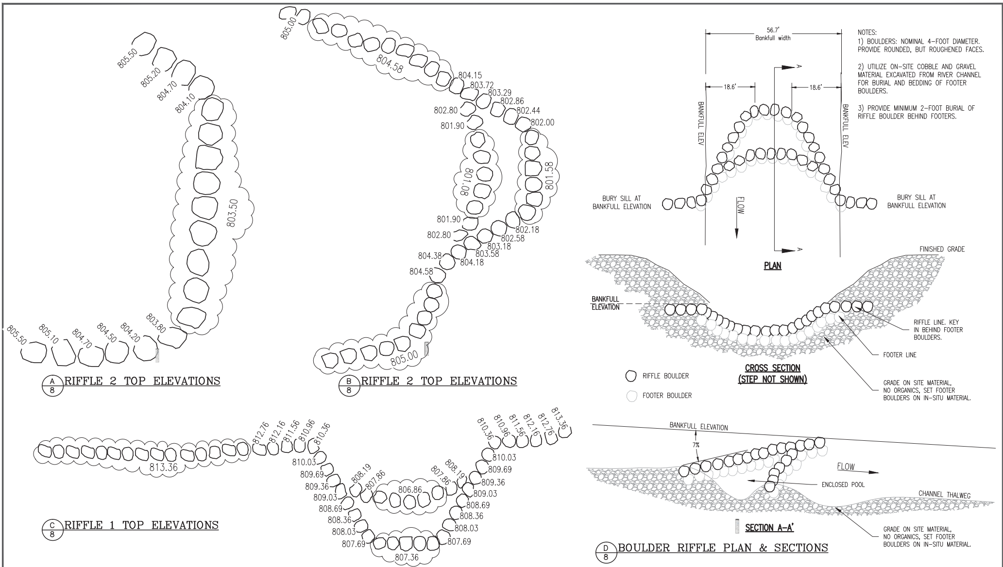
Figure 11: Riffle Details
