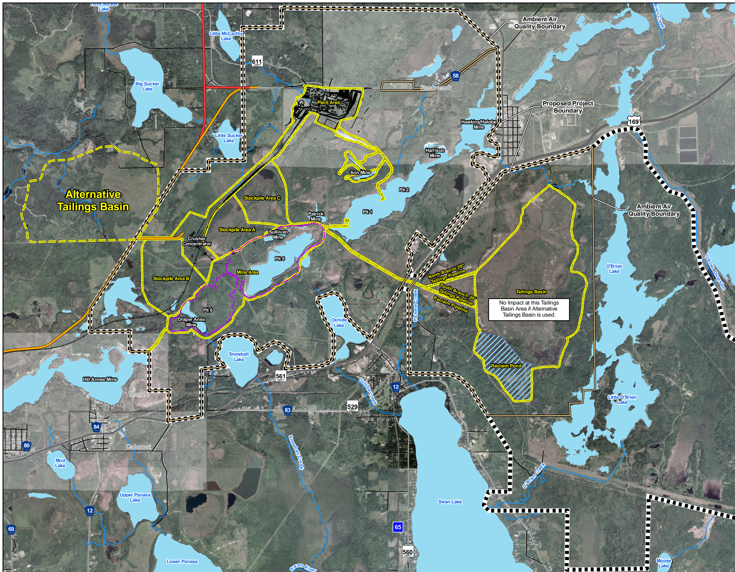
Figure 3.2 Alternative Tailings Basin Minnesota Steel Industries Nashwauk, Minnesota
