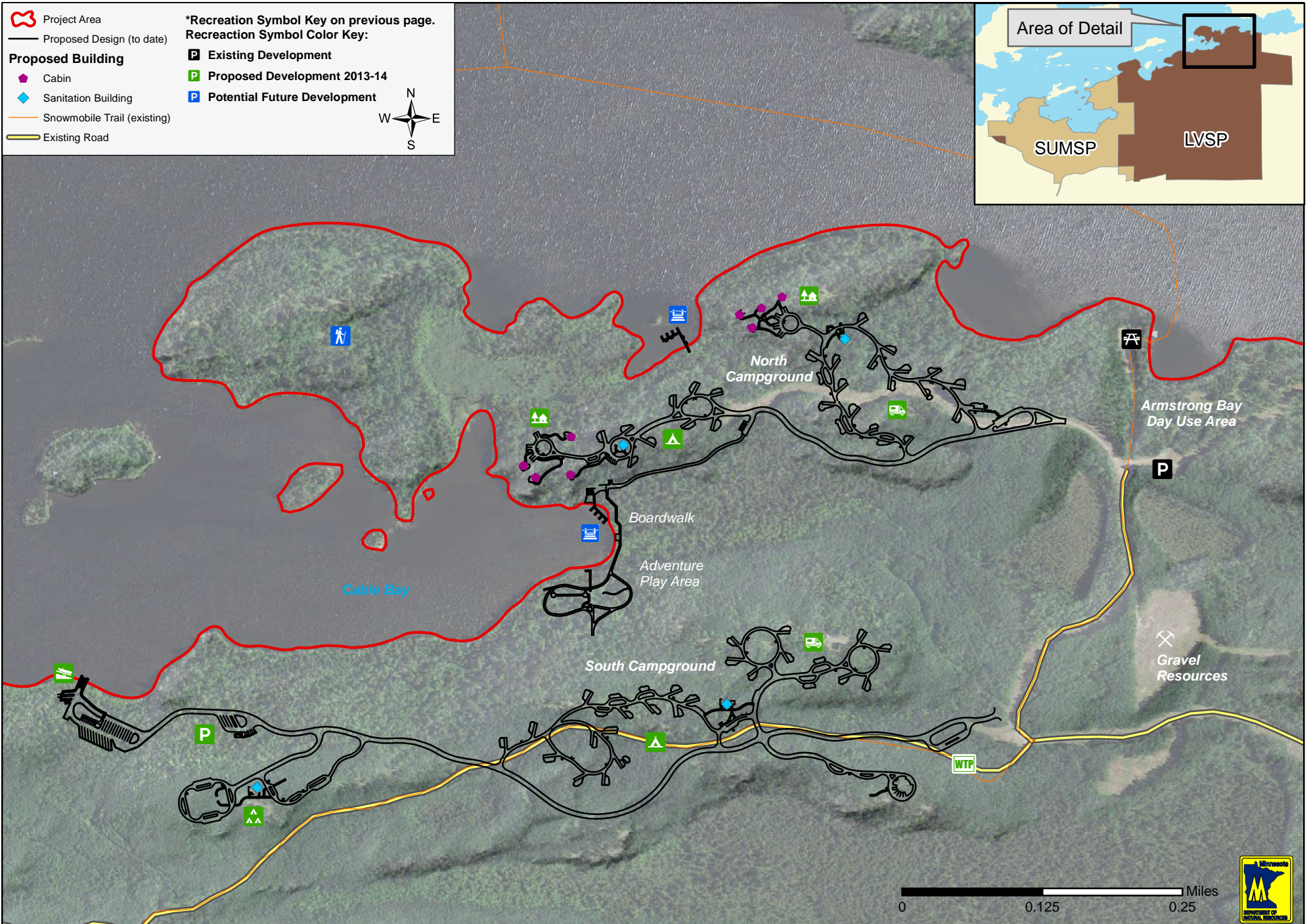
Figure 7: Lake Vermilion and Soudan Underground Mine State Parks - Proposed Concept for Main Campground Area
