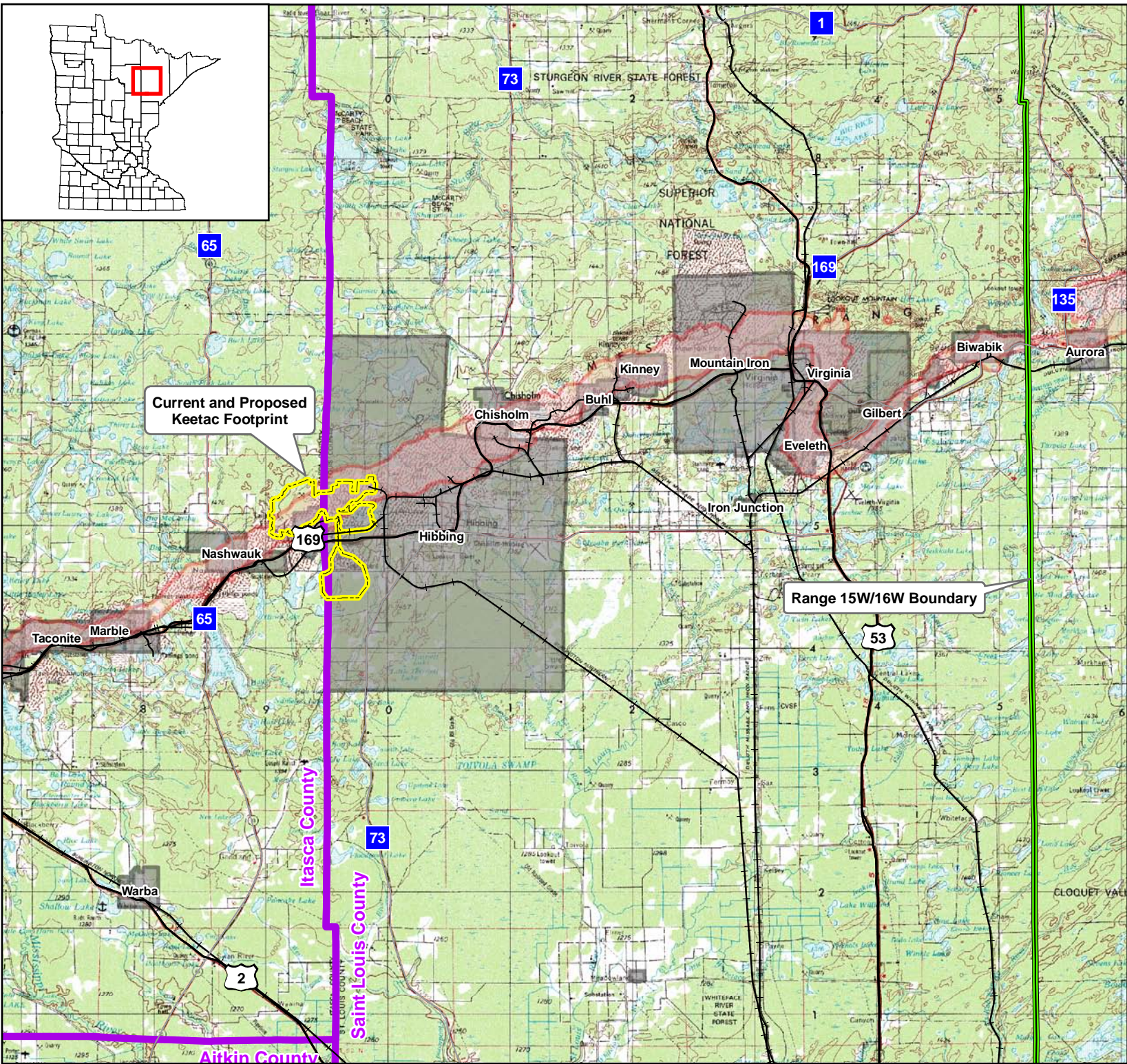
Figure 4.23.2 MndOT Tailings Acceptance Boundary U.S. Steel Keetac Keewatin, MN
