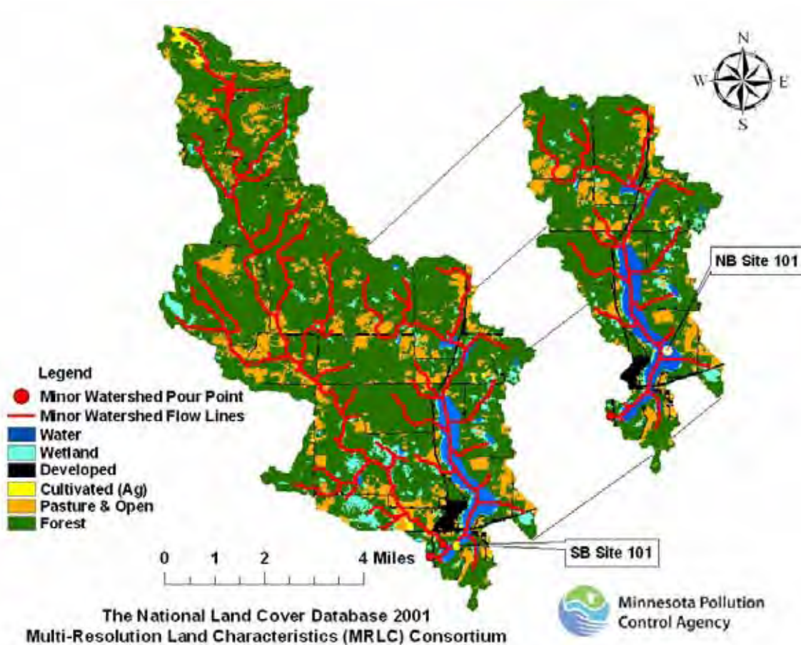
Figure 5. Hill Lake NB & SB sample locations, watershed areas, and land use composition
